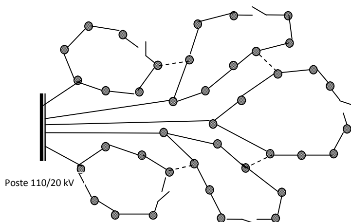
Fig.3. Structure of the networks ringed with a connection towards the node of supply; electric transformation station
