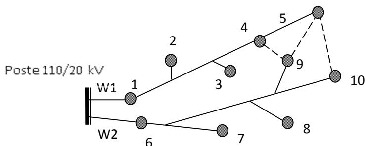
Fig.1. Emergency plugging chart between two branches supplied by a station
