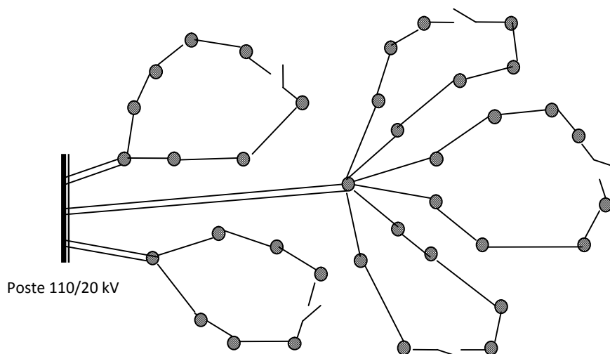
Fig.4. Structure of the networks ringed with a double connection towards the node of supply; electric transformation station
