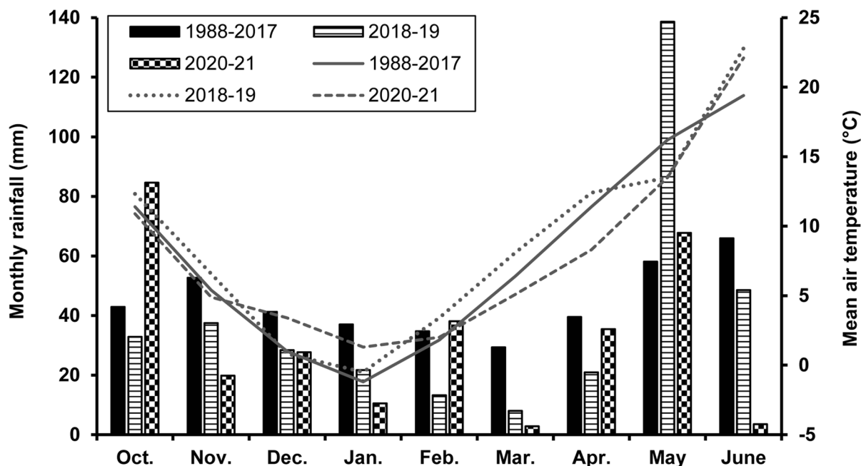
Fig. 1. Monthly rainfall (mm; columns) and mean air temperature (°C; lines) in the nursery of the Centre for Agricultural Research (Martonvásár, Hungary) during the winter wheat growing seasons. Long-term (1988–2017) average is displayed for reference.
