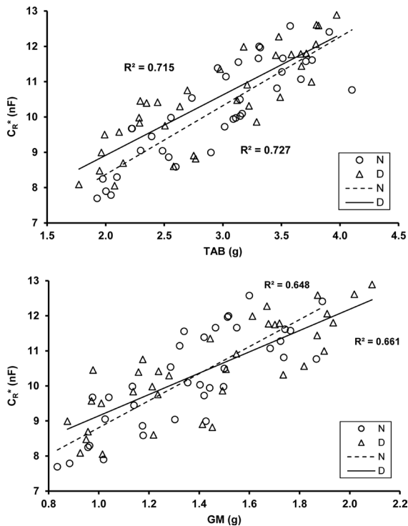
Fig. 7. Relationships between the saturation root electrical capacitance ( C_R^* ) measured at the flowering stage and the total aboveground biomass (TAB) and grain mass (GM) per plant for wheat cultivars Mv Nemere ("N") and Mv Dandár ("D") grown under low nitrogen level and ambient [CO_2] . Regressions were significant at the p < 0.001 level ( n = 36 ).
