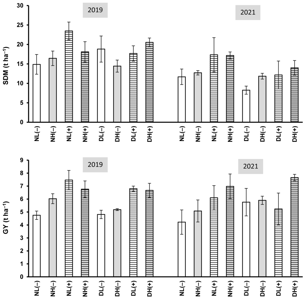
Fig. 5. Shoot dry mass (SDM) and grain yield (GY) of wheat cultivars Mv Nemere ("N") and Mv Dandár ("D") grown under low ("L") or high ("H") nitrogen supply under ambient ("−") or elevated ("+") [CO 2 ] in two years. Vertical bars represent SDs (n = 3).
