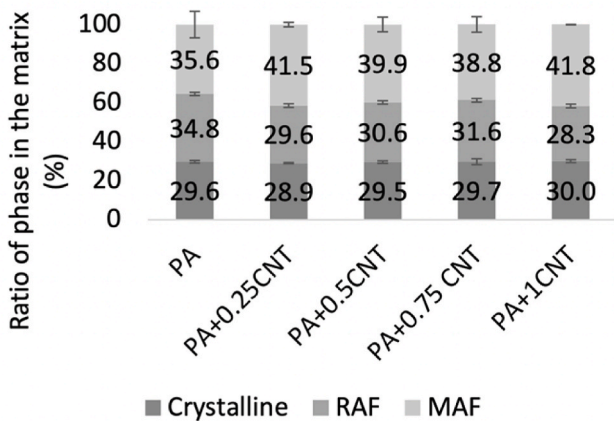
Fig. 11. Proportion of the crystalline, the rigid amorphous and the mobile amorphous fractions in the PA6 and the nanocomposites.
