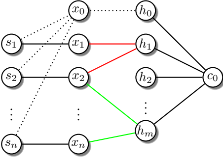
Fig. 2. Polynomial-time transformation of an arbitrary set cover instance into a corresponding instance of LHPP. In the example red and green edges represent that s_1, s_2 \in U_1 and s_2, s_n \in U_m , respectively.
