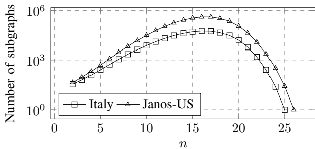
Fig. 4. The number of possible subgraphs of size n in the Italy and Janos-US networks.
