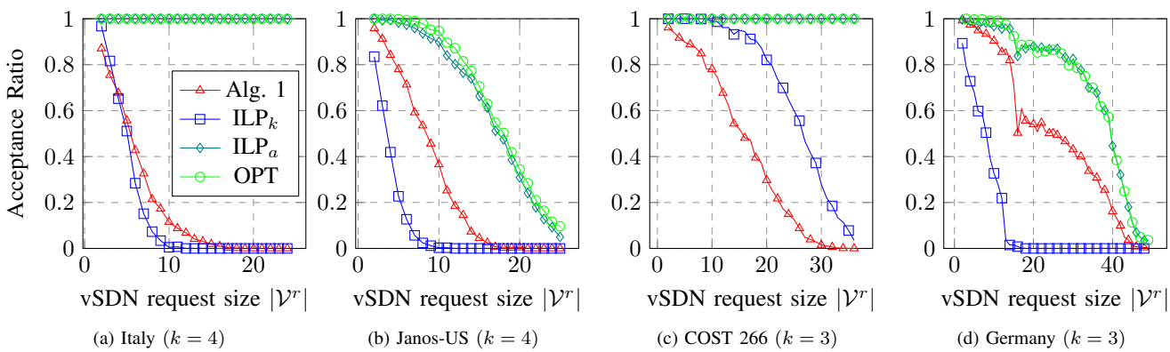
Fig. 8. Comparison about the acceptance ratio of the hypervisor placement methods in the investigated networks subject to the vSDN request size ( |\mathcal{V}^r| ) for latency requirement L = 0.6 (averages based on 10 independent runs). After each network name the number of active hypervisors ( k ) is displayed.
