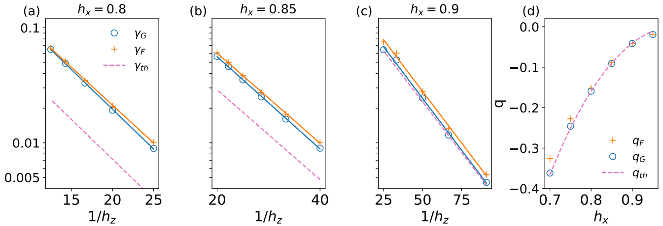
FIG. 3: Decay rates in the quantum Ising chain. In panels (a),(b),(c) we show the decay rates \gamma_F, \gamma_G , obtained from the fits of F(t), G(t) as in Fig. 2. The continuous lines are the fits of the exponential dependence of the rates in 1/h_z . The dashed line represents the theoretical prediction (6). From the fits the coefficients q_F and q_G are extrapolated and showed against the theoretical value q_{th} = |f(-i \ln h_x)|/M (dashed line) in panel (d).
