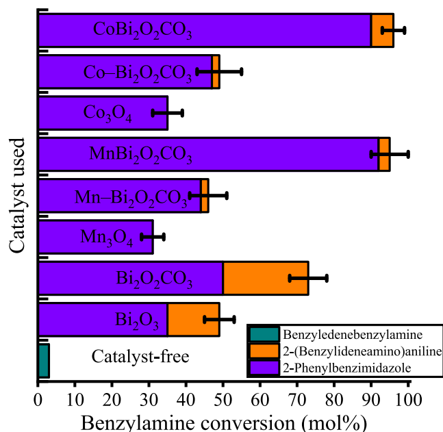
Fig. 8. The effect of the quality of the catalysts in the oxidative coupling of benzylamine and 2-aminoaniline. Reaction conditions: 1 equiv. (0.25 M) of benzylamine, 1.2 equiv. of 2-aminoaniline, DMSO:H 2 O 1:9 (2 mL), 10 mol% of catalyst, 100 °C for 24 h. (MnBi 2 O 2 CO 3 : co-precipitated samples; M-Bi 2 O 2 CO 3 : impregnated samples.)
