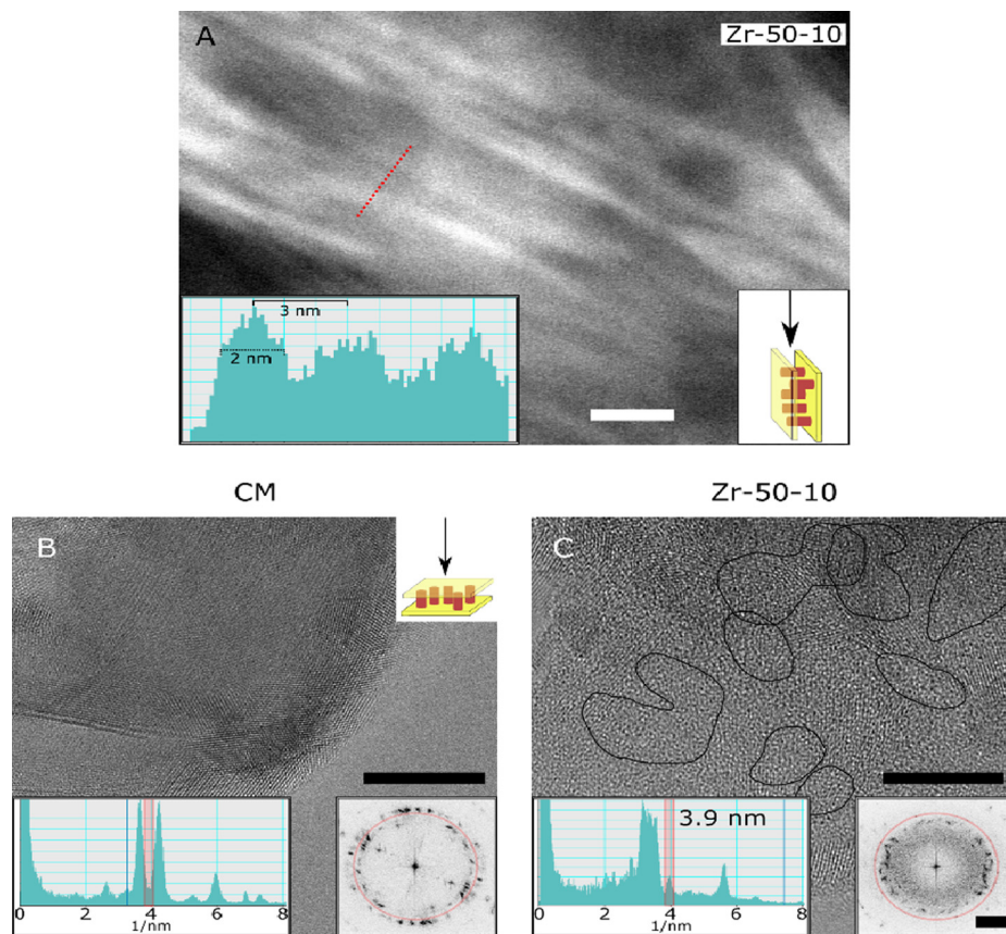
Fig. 7 HAADF image of Zr-50-10 (A) showing the presence of large \text{ZrO}_2 -domains. Representative HRTEM images of CM (B) and Zr-50-10 (C), both with their respective Fourier transforms and radially averaged Fourier transforms as insets, the red rectangle and circle indicating the peak at 3.9 \text{ 1/nm} corresponding to the [1 1 0] or [200] reflection of \text{ZrO}_2 . The scale bars in images A-C correspond to 10 nm. The scale bar in the Fourier transforms insets in B-C correspond to 2 \text{ nm}^{-1} .
