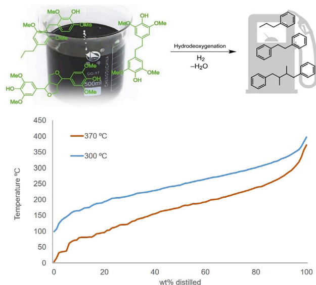
Figure 4. Hydrodeoxygenation of oligomeric fraction yields hydrocarbons in fuel range Simulated distillation curves of biofuel obtained at different HDO reaction temperatures.
