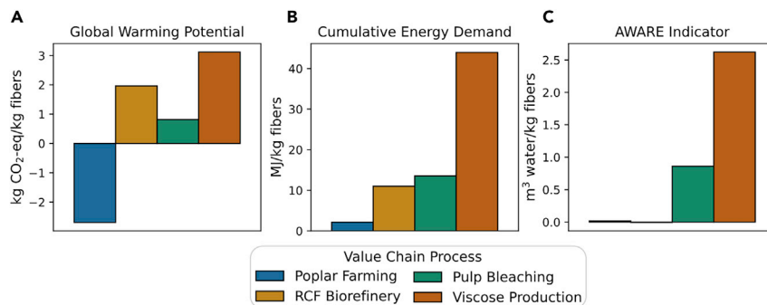
Figure 6. Life cycle impacts by the value chain process for poplar viscose fibers
