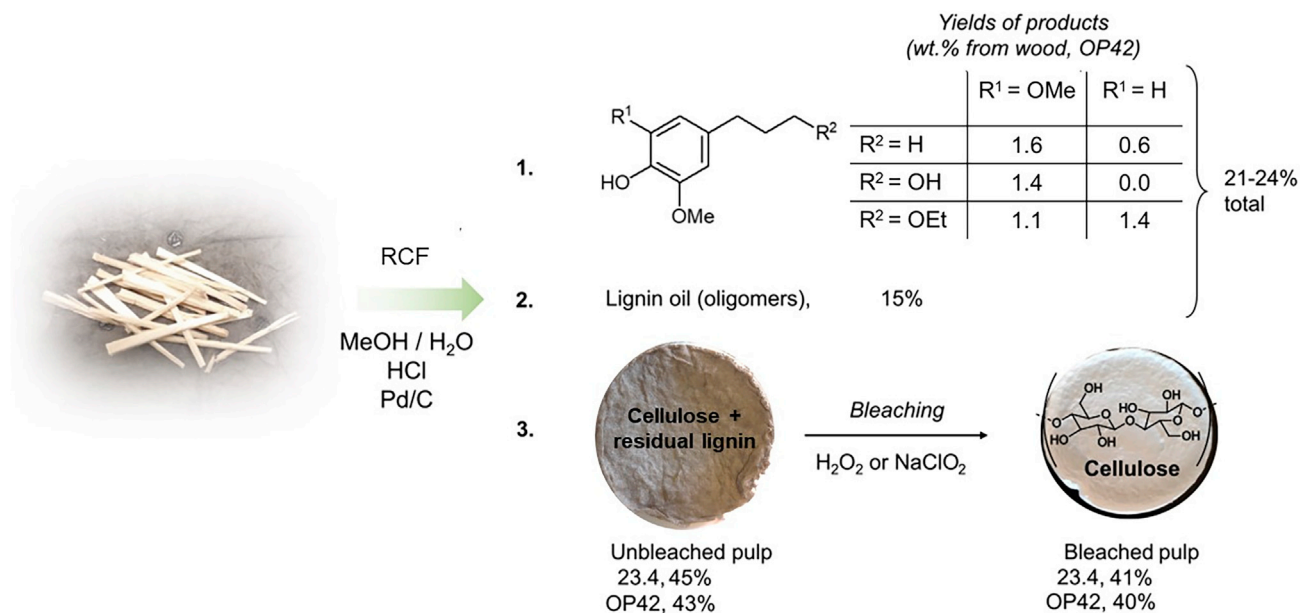
Figure 3. Catalytic fractionation of poplar wood to yield cellulose-based pulp and bio-oil
