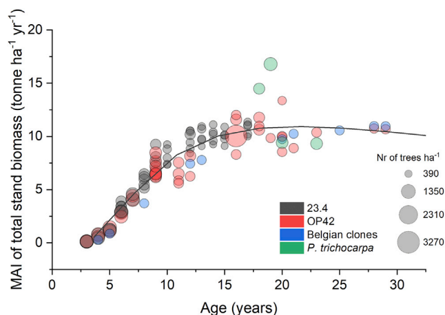
Figure 2. Mean annual biomass increment (MAI) of poplar stands measured in Sweden and Lithuania
