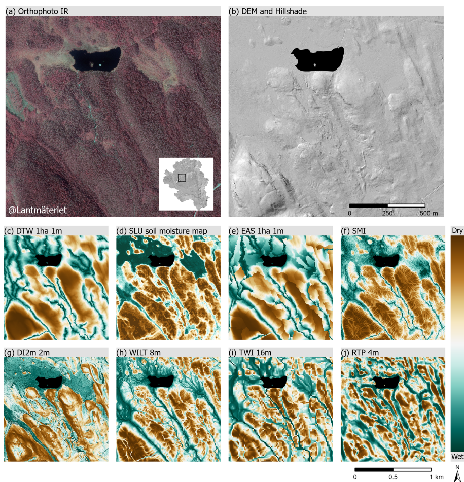
Figure 4. Orthophoto (© Lantmäteriet) (a) and hill-shaded DEM (b) covering a till area within the Krycklan catchment. Below, maps of the highest-performing maps of different terrain indices in order of VIP_{\text{predictive}} with simplified common symbology for terrain indices (c–j) based on value distribution for the visual comparison.
