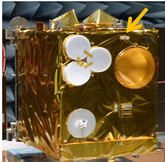
Figure 1. Photograph of Flying Laptop Satellite and the two transmitter collimators of OSIRISv1 (beneath arrow).
