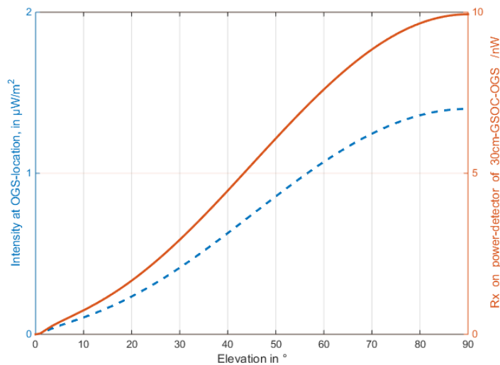
Figure 9. Calculated axial Intensity at OGSs-distance (dashed line, left axis) and optical power onto the power detector of the GSOC-OGS (solid line, right axis)
