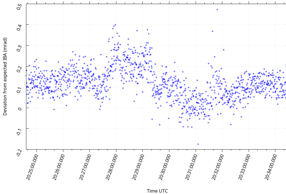
Figure 14. Deviation from expected Inter-Bore-sight Angle of the two Star Cameras, secondwise
