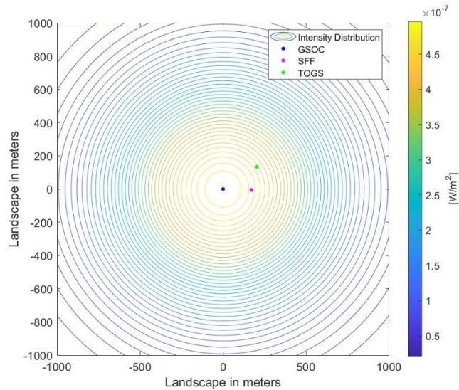
Figure 11. Theoretical Gaussian intensity distribution of FLP's optical signal at 20:27:30 UTC (25° elevation, 1203km link distance), in the perpendicular plane to the laser beam.
