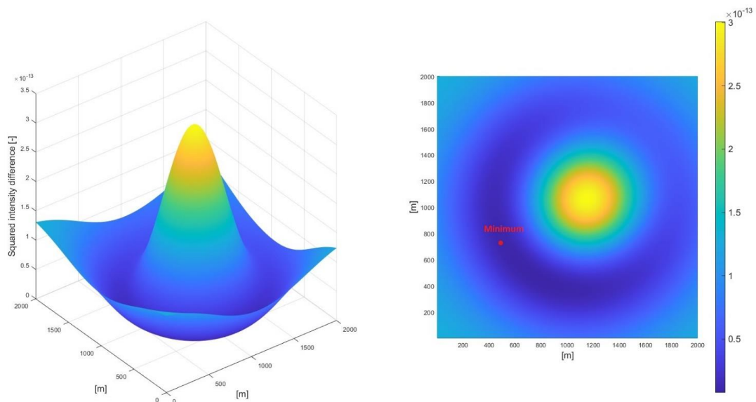
Figure 12. Comparison theoretical and measured intensity values (CoG detection)
