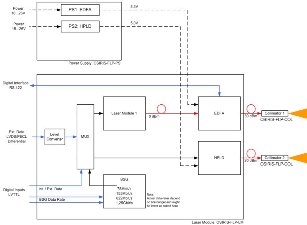
Figure 2. OSIRISv1 setup, as located onboard FLP.
