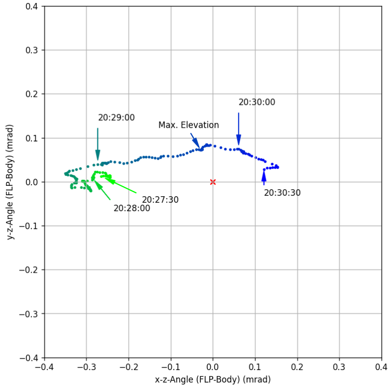
Figure 15. Plot of the pointing-error as measured by the satellite's AOCS, dots are separated by 1s.
