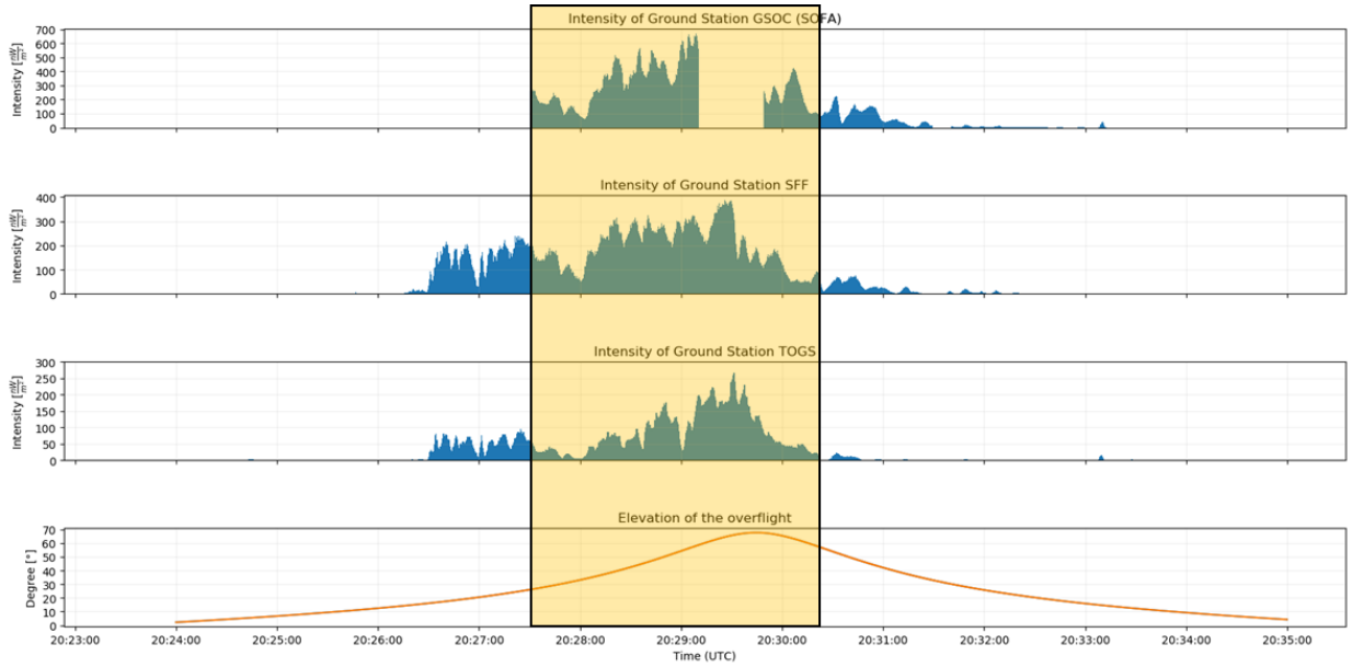
Figure 10. Intensities onto the three OGS' vs time, back-calculated from the measured received optical power. Time-window evaluated for 3OGSE is marked. Lowest plot shows the elevation over time.
