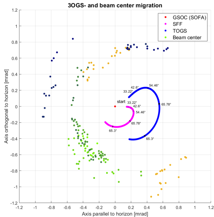
Figure 13. Run of the CoG-offset in mrad , on the plane(s) perpendicular to the laser beam, estimated from the three intensity vectors. These positions (dots) are separated by 1s each, starting with green at bottom (at 20:27:30) going to blue on top (at 20:30:20). Orange dots mark the section where intensity from only two OGS where available, resulting in 50% of the solutions appearing ambiguous at the lower right. The positions of the three OGS' can be seen with GSOC-OGS in center (red), and SFF (pink) and TOGS (blue) separated to the right, wandering by their perspective positions. Their locations are marked on their plots every 30 seconds with the according elevation.
