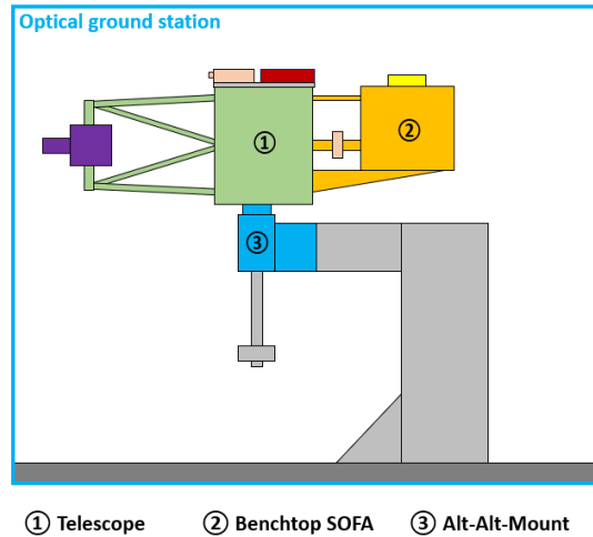
Figure 7. Schematic structure of the 30cm optical ground located at GSOC.
