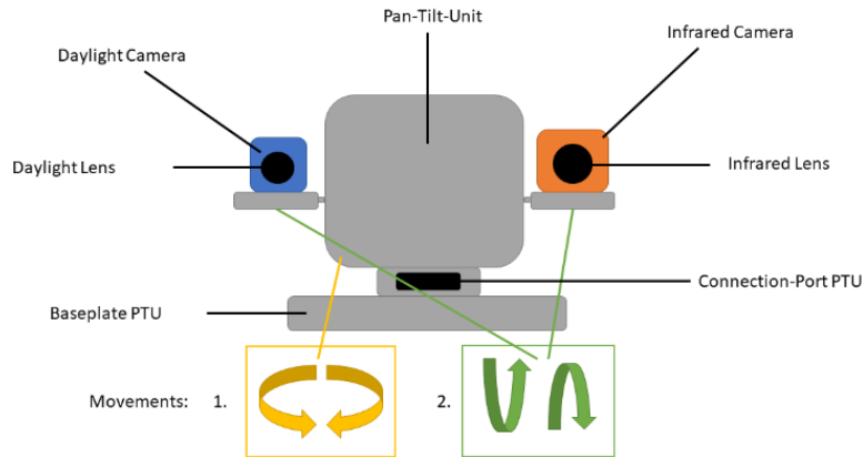
Figure 5. Functional diagram of the Satellite Flash Finder.
