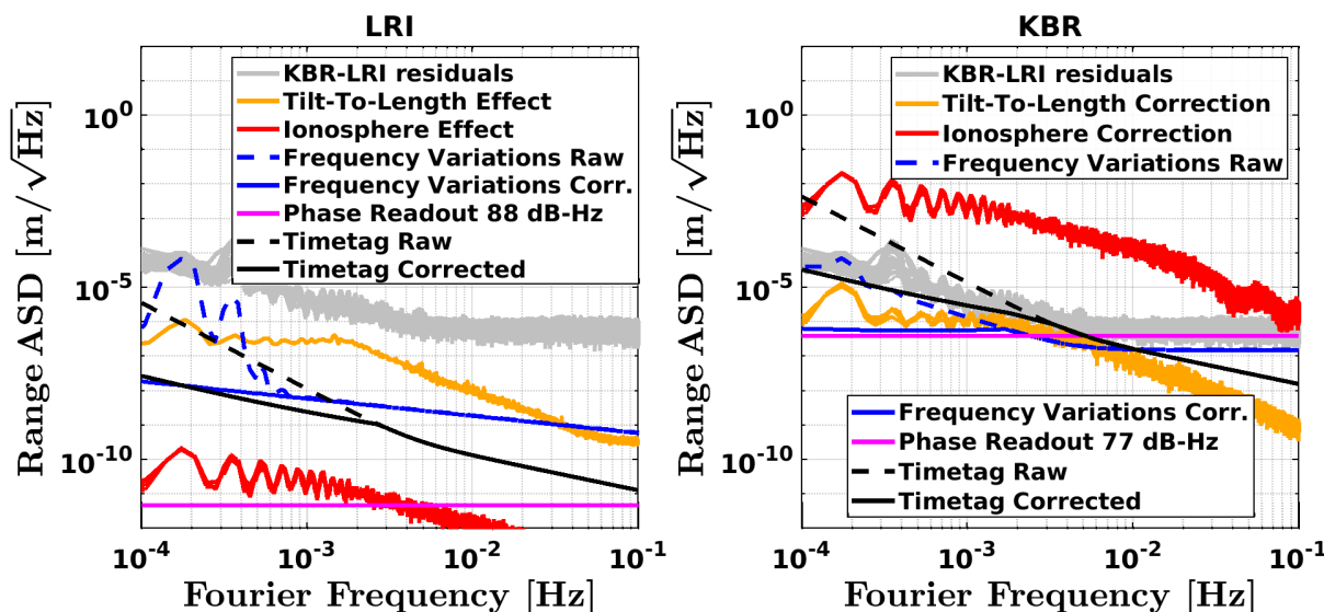
Figure 4. Noise contributors and corrections in LRI and KBR in terms of amplitude spectral densities (ASDs). The grey KBR-LRI residuals are described in Section 5 and replotted from Figure 3. The KBR tilt-to-length correction (Antenna-Offset-Correction) in orange is provided in the KBR1B dataset and already removed in the KBR range, while the corresponding effect in the LRI has a lower magnitude and was derived based on [38]—see Section 6.2 for more details. The ionospheric correction (red) is relevant for KBR, but negligible in LRI due to the scaling with wavelength. The smaller wavelength of the laser scales the phase readout noise (magenta) to a negligible level as well, while in KBR, it is dominant at high frequencies (cf. Section 6.3). Raw frequency variations (dashed blue) assume a static frequency (within one day) and are related to the stability of the optical cavity and proper time effect in the LRI, whereas they are related to the USO stability in KBR. These raw frequency variations can be corrected by using a time-dependent frequency (cf. Section 6.5). The effect of timetag errors is being corrected in LRI and KBR by employing CLK1B \epsilon_{\text{time}} information (dashed vs. solid black traces). For some legend entries, multiple days were plotted in order to illustrate the stationarity and variability of the traces. The mean satellite separation is L = 194 km for January 2019. The ENBW for both plots is 52 \mu\text{Hz} .
