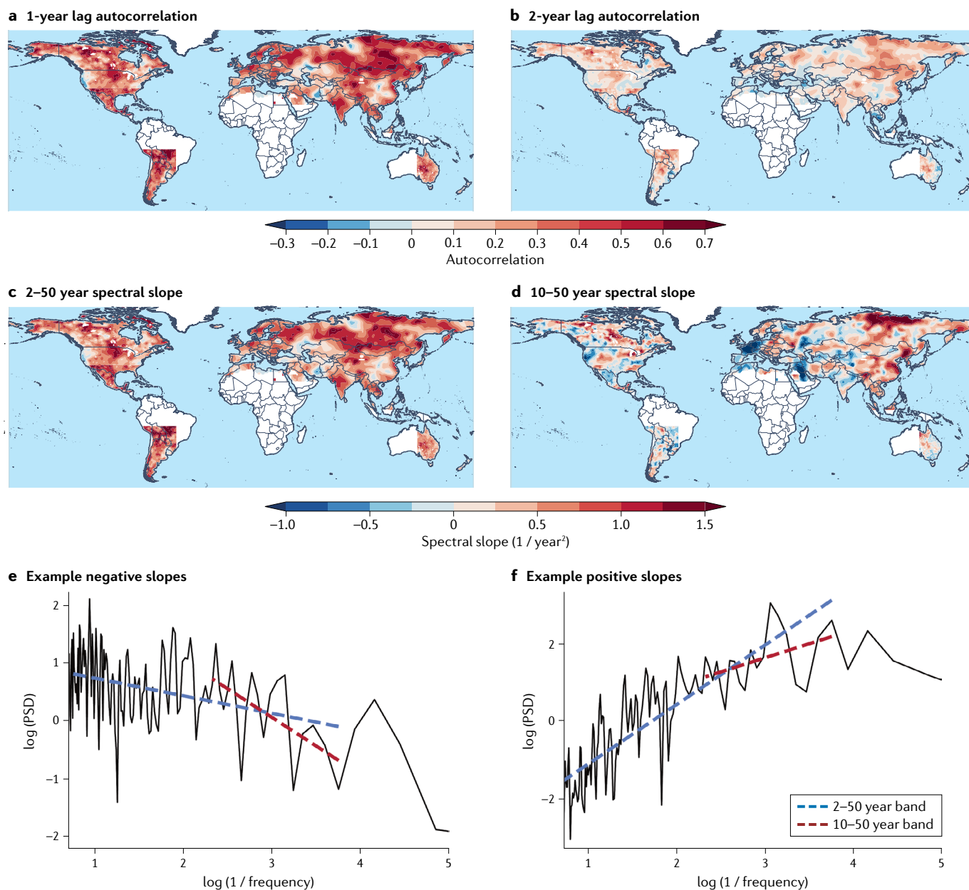
Fig. 1 | Common Era drought characteristics of soil moisture. a,b | Autocorrelation (unitless) of the tree ring-derived drought atlas Palmer Drought Severity Index (PDSI) for 1400–2000 Common Era (CE) at 1 and 2-year lags. c,d | Slopes ( 1/\text{year}^2 ) of PDSI power spectral density (PSD), filtered for periodicities of 2–50 years and 10–50 years. Slopes calculated using a least squares regression of the log-transformed power spectral density against the log-transformed periodicity ( 1/\text{frequency} ). e,f | Examples of grid cells with large negative and positive power spectral slopes, with those of the 2–50 year band (blue) and the 10–50 year band (red). Data over
