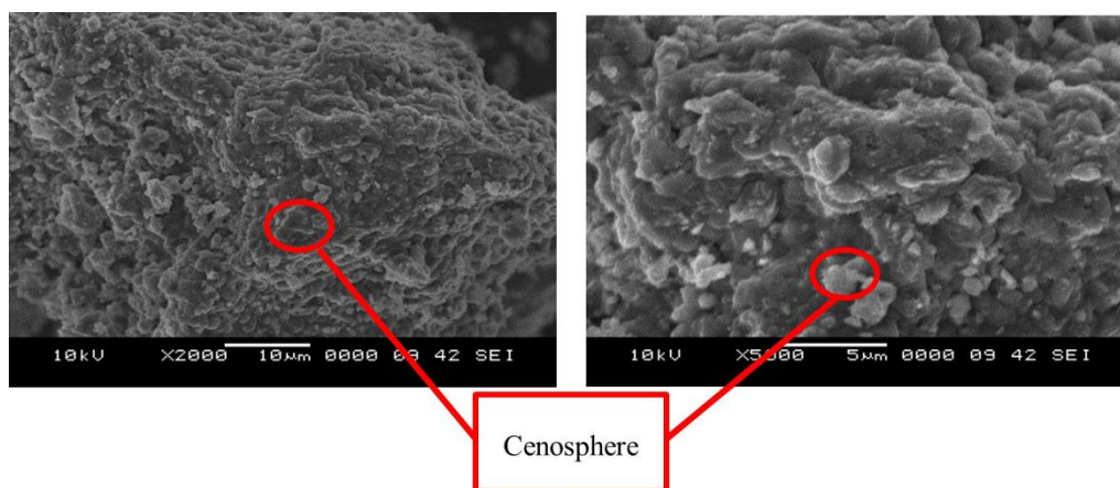
Figure 7. SEM micrographs of the high calcium pozzolanic-based geopolymer at 2000× and 5000× magnification.
