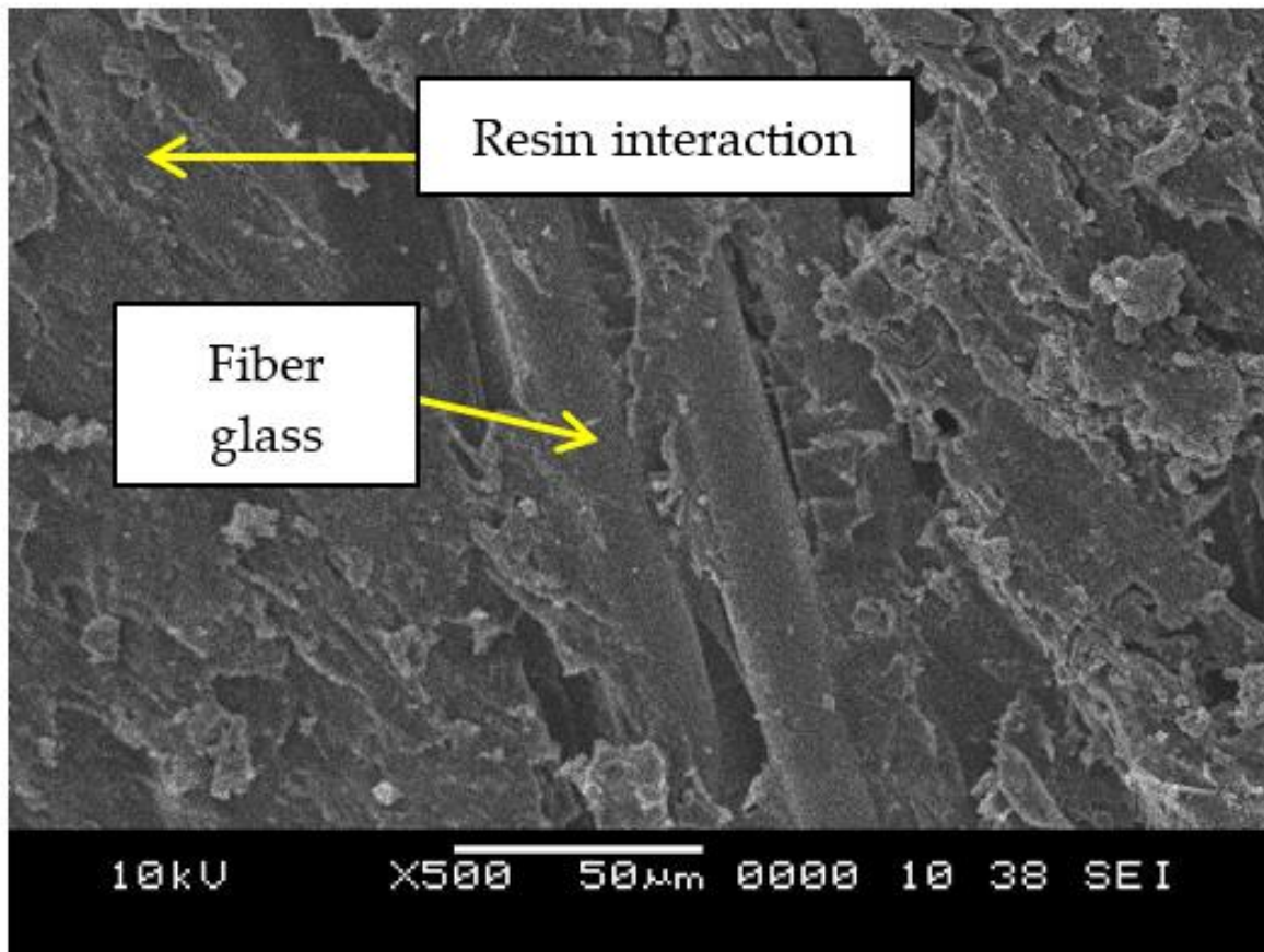
Figure 10. SEM images of control sample GRE pipe without any geopolymer filler.
