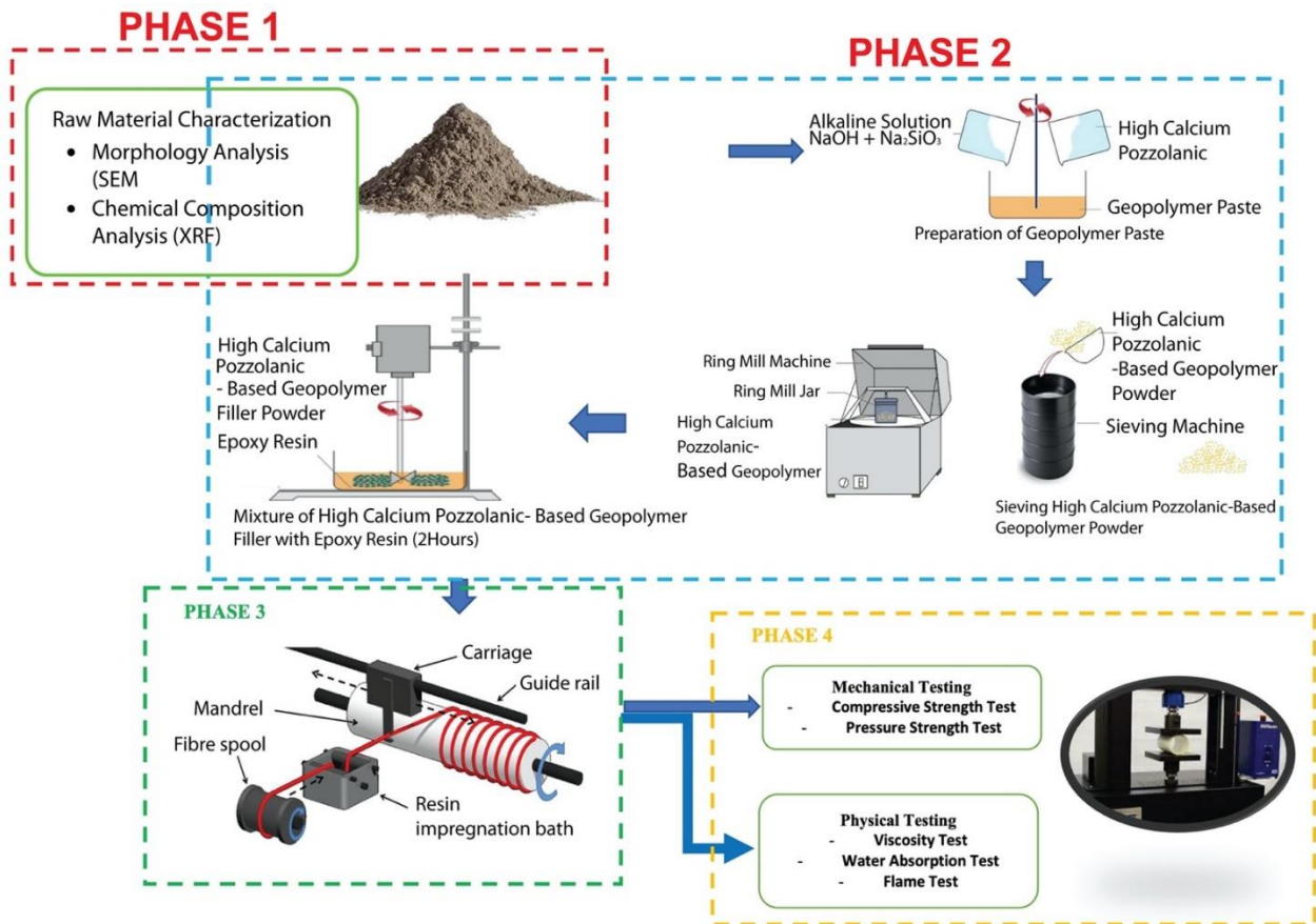
Figure 2. Process flow of the product development and characterization for epoxy filled with geopolymer composite pipe via filament winding.
