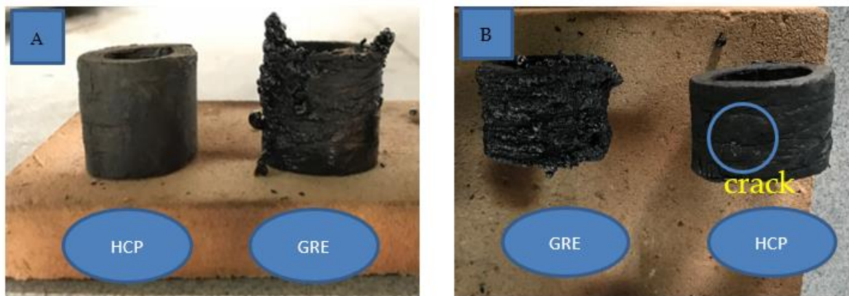
Figure 14. Heat resistance properties of (A) horizontal and (B) vertical of GRE pipe with high calcium pozzolanic-based geopolymer filler and GRE without geopolymer filler.
