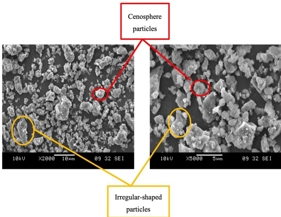
Figure 6. SEM micrographs of the raw high calcium pozzolanic at 2000× and 5000× magnification.
