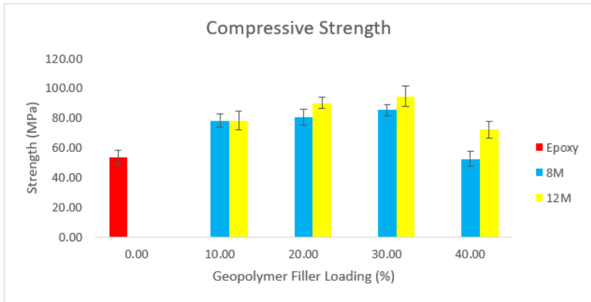
Figure 12. Compressive strength of GRE pipe with 0–40 wt% geopolymer filler loading.
