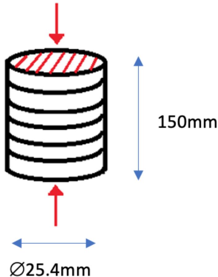
Figure 3. Schematic diagram of testing pipe sample on vertical position.
