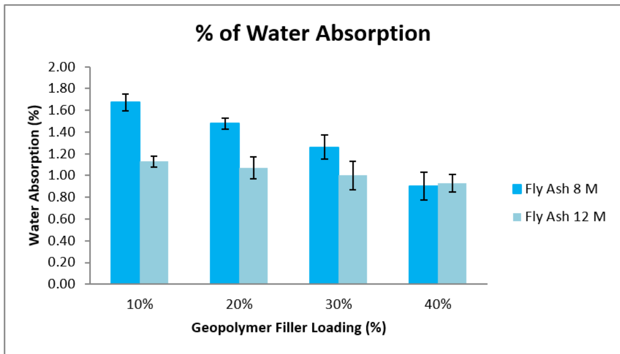
Figure 9. Comparison graph of % water absorption between samples.
