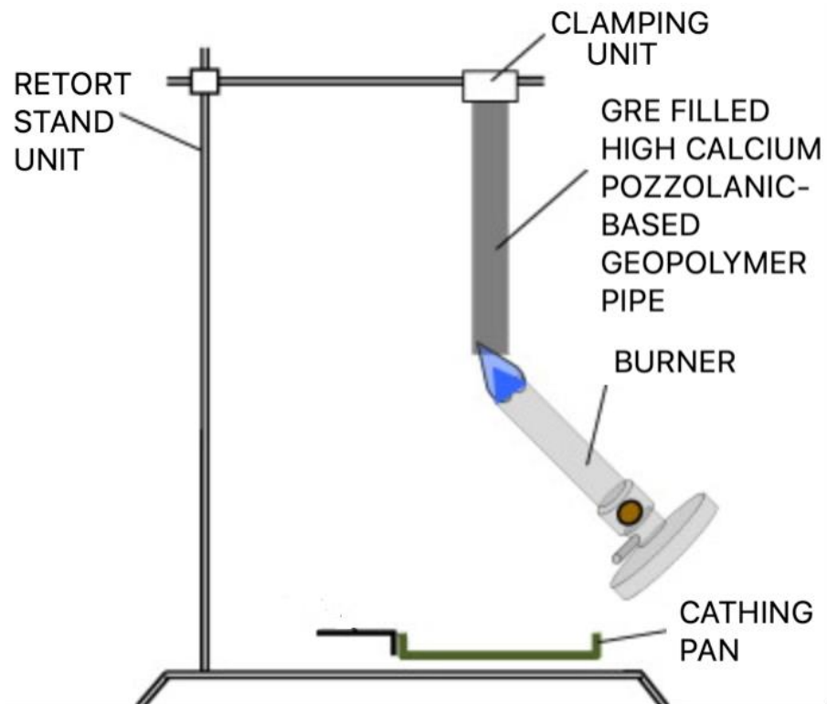
Figure 4. Schematic diagram of flame test.
