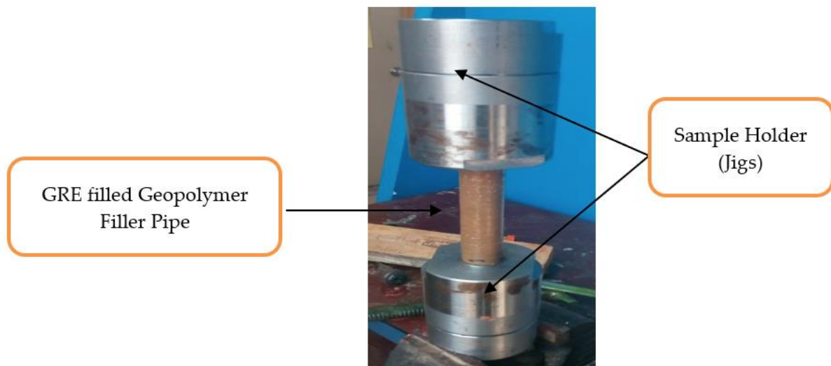
Figure 5. Hydrostatic pressure leak test.
