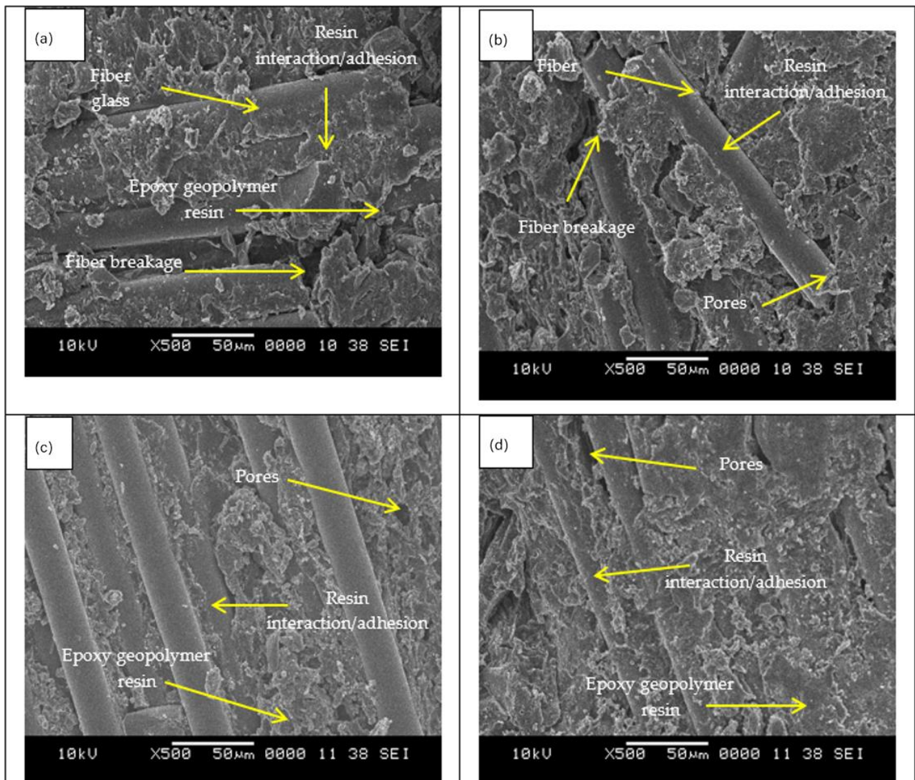
Figure 11. SEM images of GRE-filled high calcium pozzolanic-based geopolymer filler pipe (a–d) with different wt% of filler loading. (a) 10 wt%, (b) 20 wt%, (c) 30 wt%, (d) 40 wt%.
