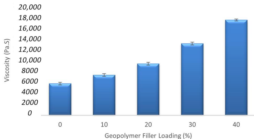
Figure 8. Comparison graph of liquid viscosity between samples.
