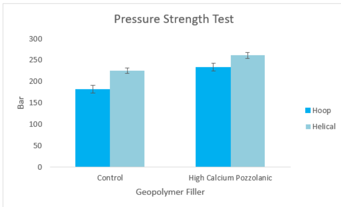
Figure 13. Burst test of the control sample and GRE filled with high calcium pozzolanic-based geopolymer pipe.
