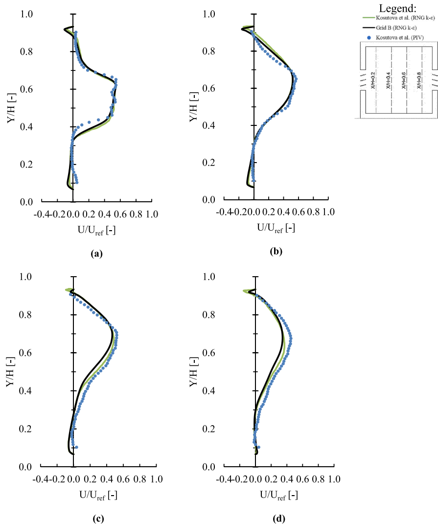
Fig. 7. Model validation of the reference grid with Kosutova et al. (Kosutova et al., 2019)'s PIV and RNG k- \epsilon for locations (a) X/H = 0.2 (b) X/H = 0.4 (c) X/H = 0.6 and (d) X/H = 0.8 .
