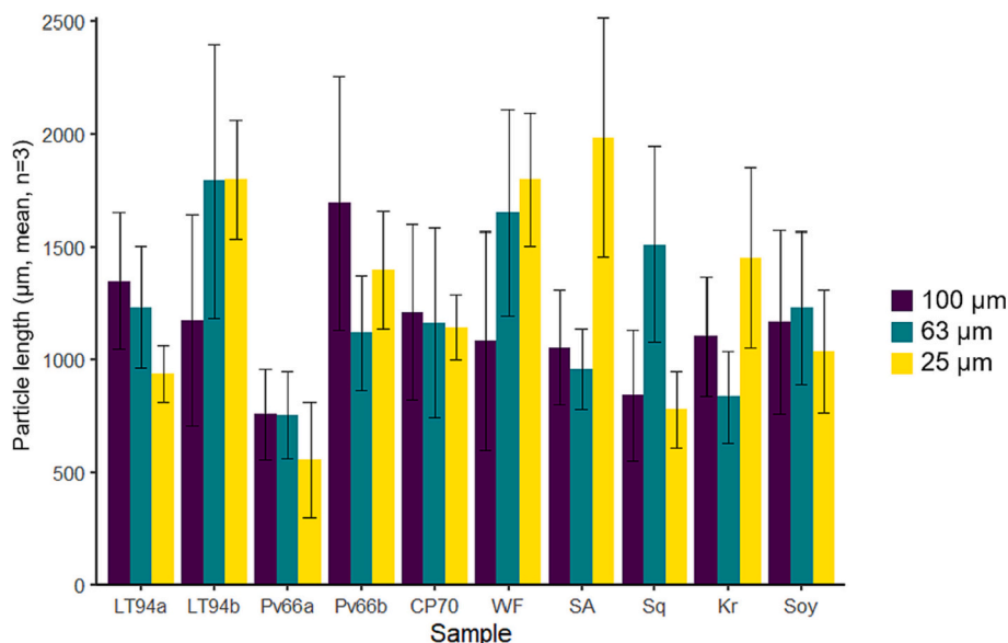
Fig. 3. Mean length of particles (calculated as largest dimension in μm) identified on 100, 63 and 25 μm pore size filters for each sample (n = 3, error bars = standard error). Refer to Table 1 for detail on aquaculture feeds.
