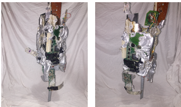
Figure 1: Two sides of the early form of the sculpture, to be positioned at the center of the space. The holes on the surface host the ultrasonic distance sensors
