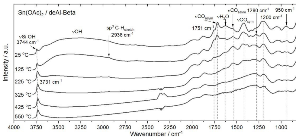
Figure 6. In situ DRIFTS for calcination of \text{Sn}(\text{OAc})_2/\text{deAl-Beta} (10 wt. % Sn) during the ramping stage.
