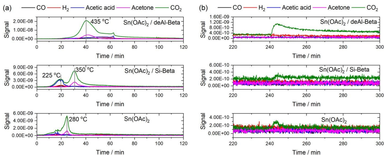
Figure 4. TPD-MS during calcination of (from top to bottom) i) Sn(OAc) 2 /deAl-Beta, ii) Sn(OAc) 2 /Si-Beta, and iii) pure Sn(OAc) 2 . (a) TPD-MS plots of the first 2 hours which includes the initial ramp from room temperature to 550 °C and part of the N 2 isotherm. (b) TPD-MS plots of the N 2 /air switch step, following the 3 h isotherm in N 2 at 550 °C.
