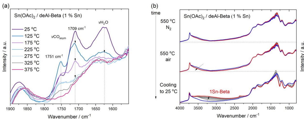
Figure 10. DRIFT spectra during heat treatment of Sn(OAc) 2 /deAl-Beta mixture with 1 wt. % of Sn (a) at different stages of the ramp rate in N 2 (zoom on CO asym bands) and (b) different steps of the isotherms and cooling to room temperature.
