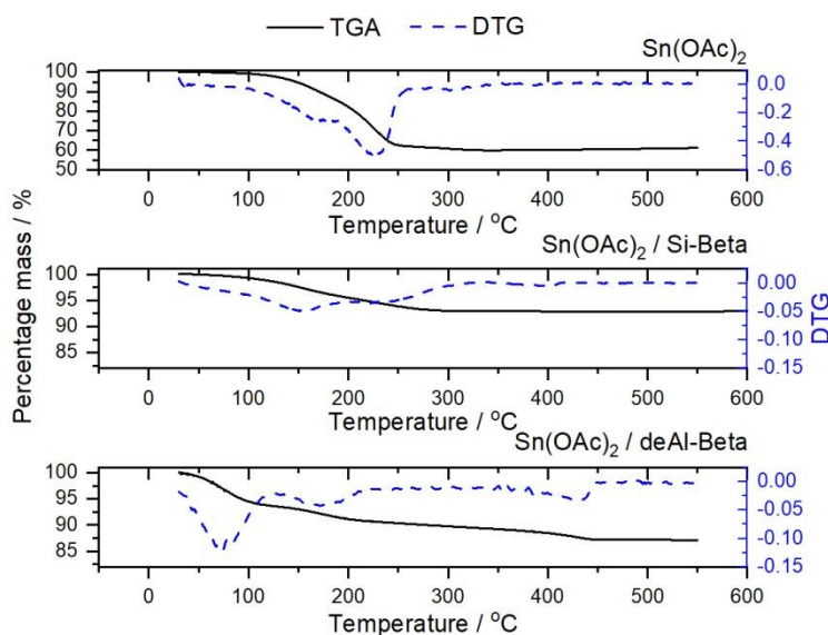
Figure 5. TGA profiles and derivatives of (from top to bottom) i) pure \text{Sn}(\text{OAc})_2 , ii) \text{Sn}(\text{OAc})_2/\text{Si-Beta} , and iii) \text{Sn}(\text{OAc})_2/\text{deAl-Beta} .
