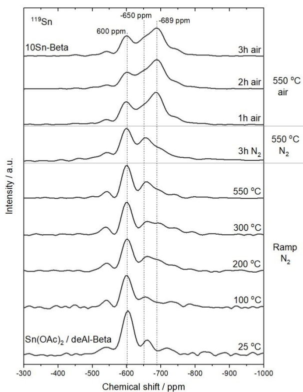
Figure 9. 119 Sn MAS DE CPMG NMR spectra of 10Sn-Beta at different stages of the ramping period in N 2 , and at different stages of the isotherm periods.
