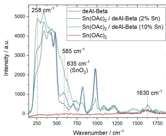
Figure 3. UV-Raman spectra of i) deAl-Beta (black line), ii) pure Sn(OAc) 2 (red line), and Sn(OAc) 2 /deAl-Beta mixture with iii) 2 wt. % of Sn (blue line), and iv) 10 wt. % of Sn (green line).
