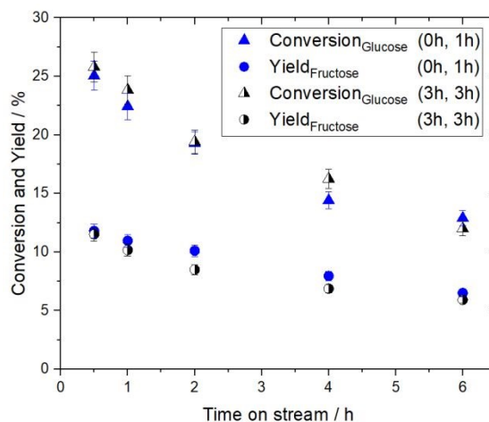
Figure 12. Continuous glucose isomerisation on 10Sn-Beta (0h, 1h) (blue symbols) and 10Sn-Beta (3h, 3h) (black symbols). Reaction conditions: 1 wt. % glucose in methanol employed as feed solution, 100 mg of catalyst packed into a stainless steel \frac{1}{4} " tube with quartz wool, 110 °C, flow rate of 1 mL min -1 .
