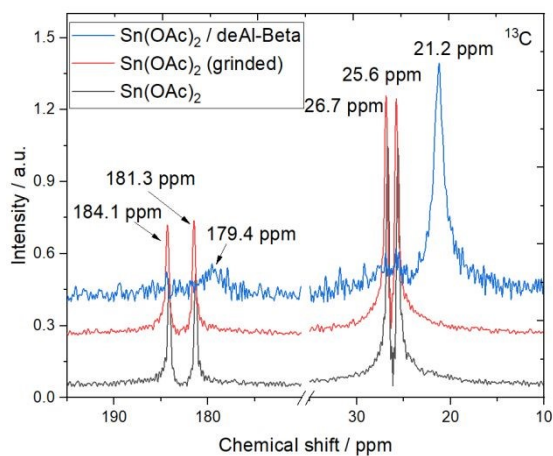
Figure 1. ^{13}\text{C} MAS NMR of untreated and grinded \text{Sn}(\text{OAc})_2 , and the grinded \text{Sn}(\text{OAc})_2/\text{deAl-Beta} mixture.
