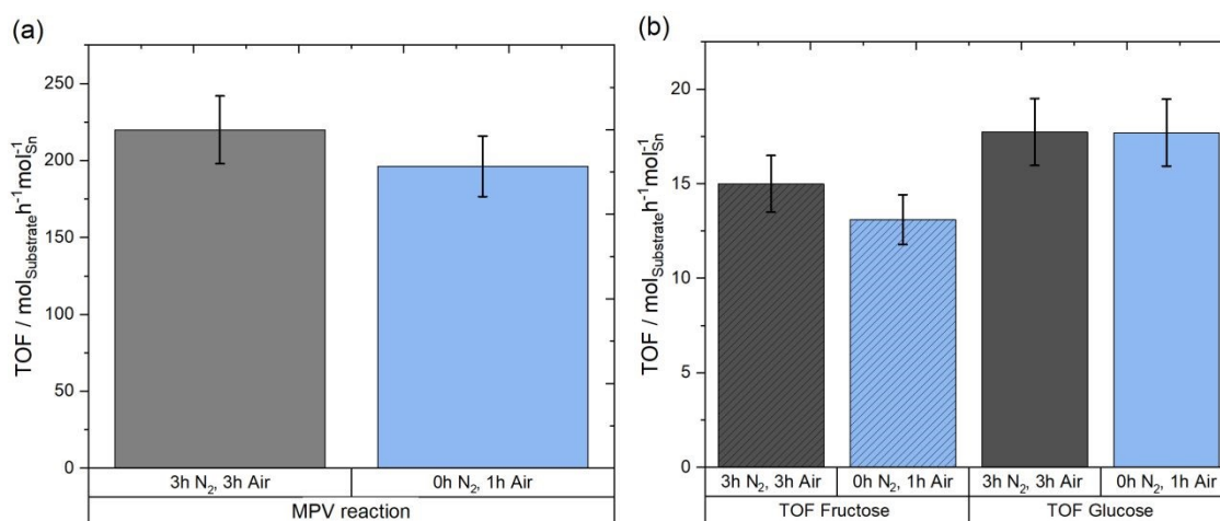
Figure 11. (a) TOF at 5 min for MPV reaction of cyclohexanone to cyclohexanol over conventional (3h, 3h) and rapidly synthesised (0h, 1h) 10Sn-Beta. Reaction conditions: 10 mL solution of 0.2 M cyclohexanone and 0.01 M Biphenyl in 2-butanol, 1:100 Sn:cyclohexanone molar ratio, 100 °C. (b) TOF for batch glucose isomerisation at 5 min over conventional (3h, 3h) and rapidly synthesised (0h, 1h) 10Sn-Beta. Reaction conditions: 5 mL of 1 wt. % glucose in methanol solution, 1:50 Sn:glucose molar ratio, 110 °C.
