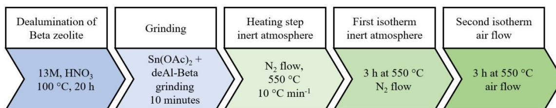
Scheme 1. Schematic of the Solid-State Incorporation (SSI) procedure.
