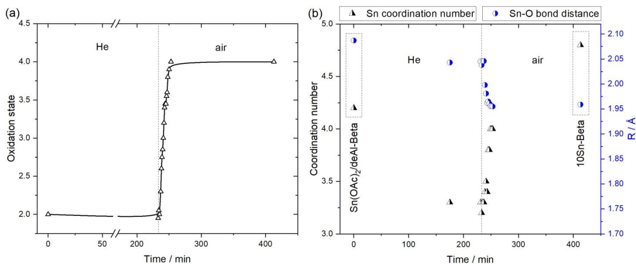
Figure 7. In situ XAS analysis of 10Sn-Beta synthesis. (a) Oxidation state of Sn as a function of time. (b) Coordination number of Sn and first-shell Sn-O bond distance obtained from XANES fitting data (further details are reported in SI Table S2).
