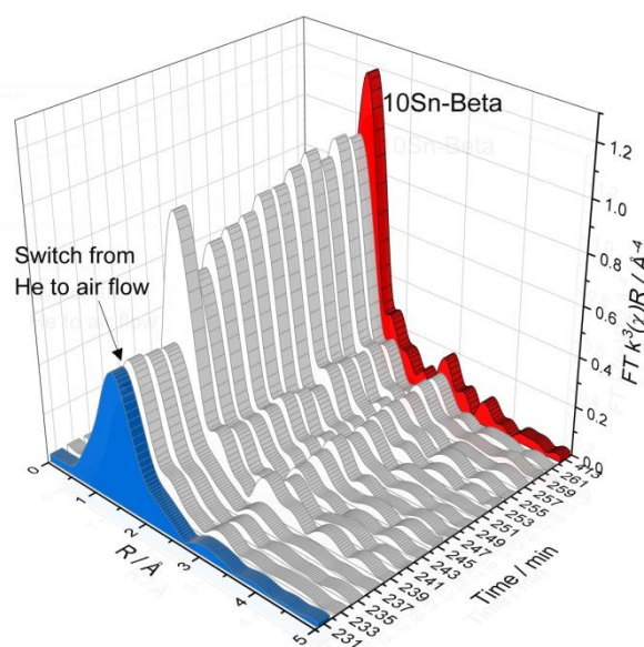
Figure 8. EXAFS 3D spectrum of the k^3 weighted FT of 10Sn-Beta calcination in R-space.
