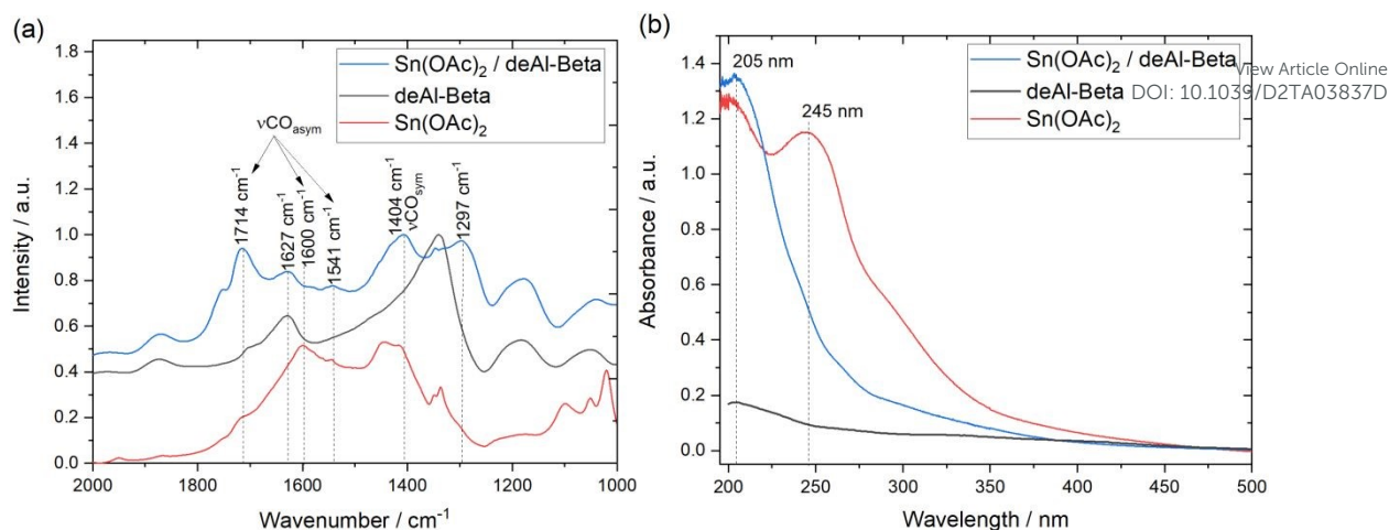
Figure 2. (a) DRIFTS comparison of deAl-Beta, Sn(OAc) 2 (grinded), and physical mixture Sn(OAc) 2 /deAl-Beta. (b) DRUV-vis spectra of deAl-Beta, Sn(OAc) 2 (grinded), and physical mixture Sn(OAc) 2 /deAl-Beta.
