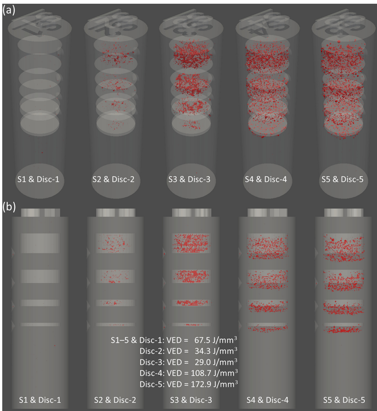
Fig. 10. Visualization of pores in samples S1-S5. (a) 3D view (b) view parallel to XZ-plane.
