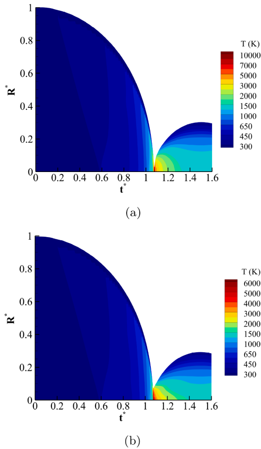
Fig. 3. Spatio-temporal contours of temperature change during the bubble collapse obtained with: (a) IG and (b) RKPR EoSs.
