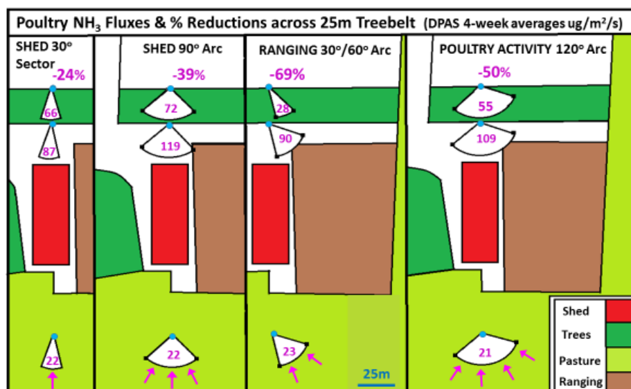
Figure 27: Poultry ammonia fluxes (ug/m 2 /s) and percentage reductions across 25m of trees for 4 transects at the 6000-bird shed: 4-week-averages for individual and combined 30° sectors from DPAS sampling
