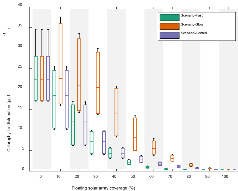
Figure 4 - Total chlorophyll- a (based on the mean of a window, \pm five days, around the day of maximum total chlorophyll- a ) versus floating solar array coverage. Whiskers represent the minimum and maximum of the simulation results presented. The box represents the 2.5 th & 97.5 th percentiles, which gives a 95% confidence interval that simulation estimates fall within this range. 0 % floating solar coverage represents QEII reservoir simulated as a baseline.
