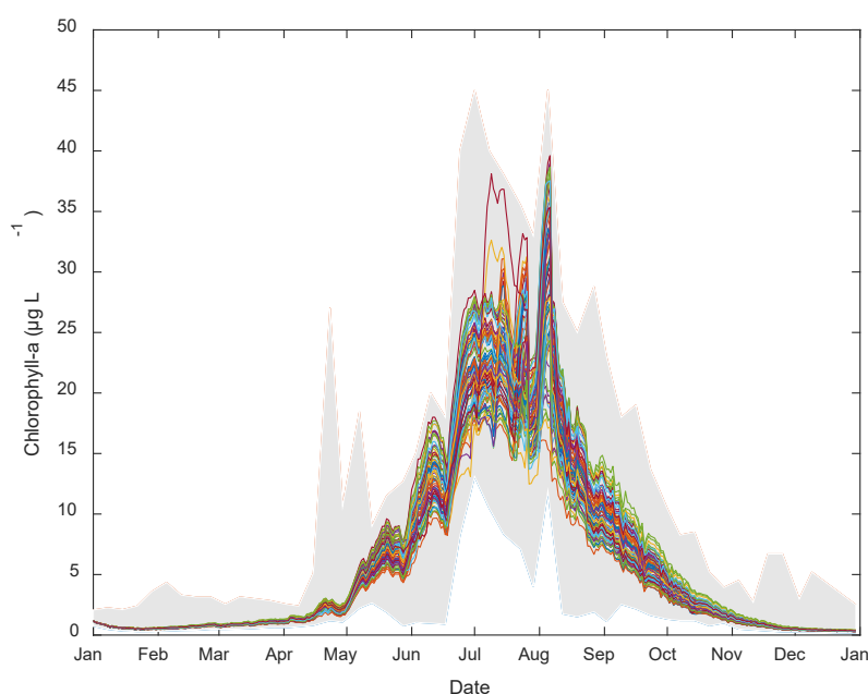
Figure 2 – Simulated chlorophyll- a (coloured lines) samples within the limits of acceptability (grey shaded area).
