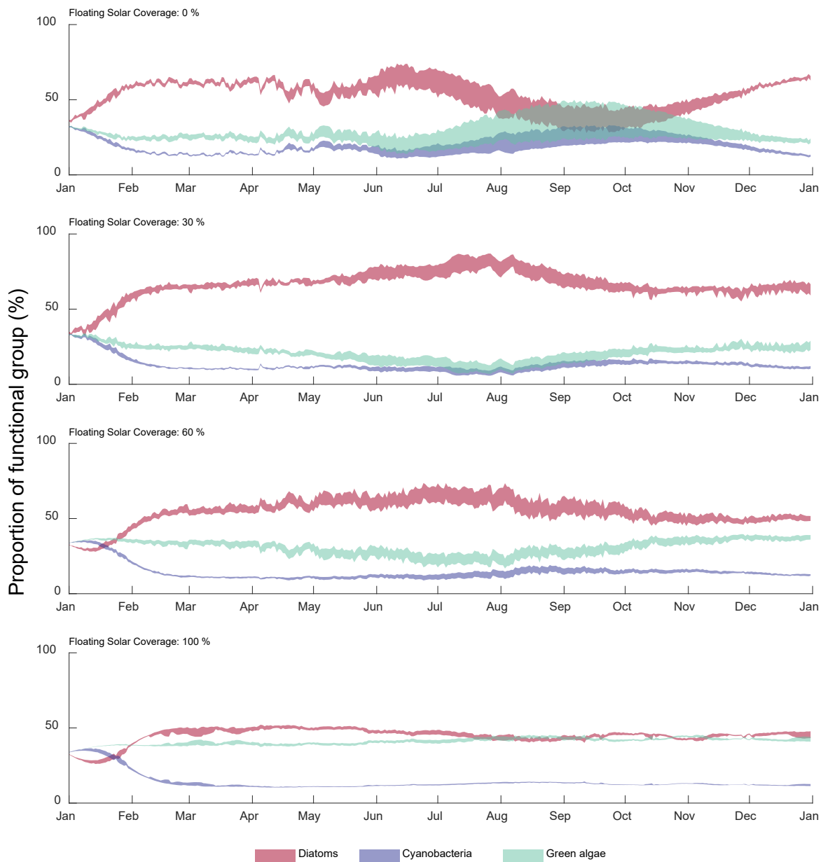
Figure 6 – Scenario-Fast: Proportion of phytoplankton functional groups as a percentage of total chlorophyll-a for the simulated period. The initial phytoplankton functional group proportions were set evenly, therefore, the first 30 days of simulations are model run-in time and should be ignored. 0% floating solar coverage represents QEII reservoir simulated as a baseline.
