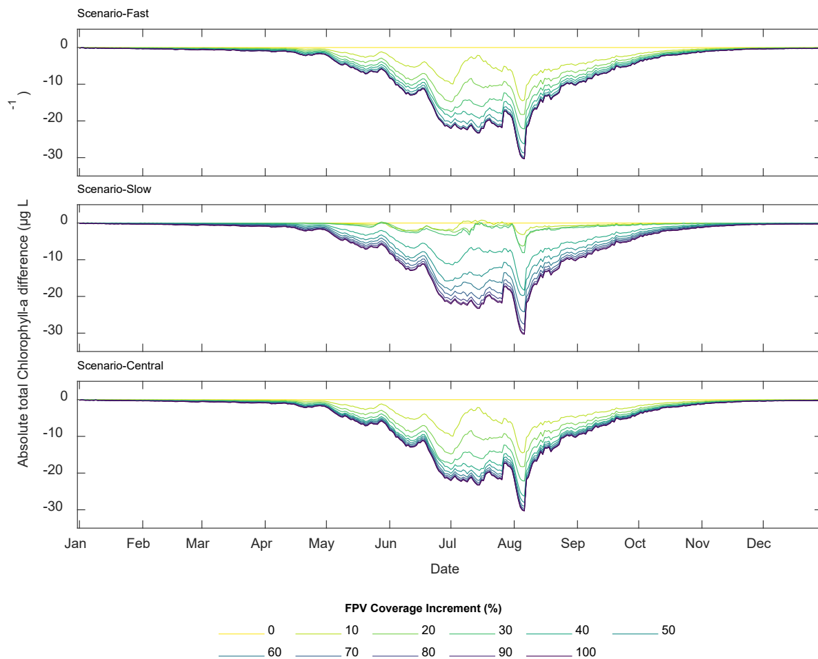
Figure 5 – Annual median total chlorophyll- a absolute difference by scenario. 0 % floating solar coverage represents QEII reservoir simulated as a baseline with no additional floating solar coverage. The relative difference in chlorophyll- a is shown in Figure S 7-1.
