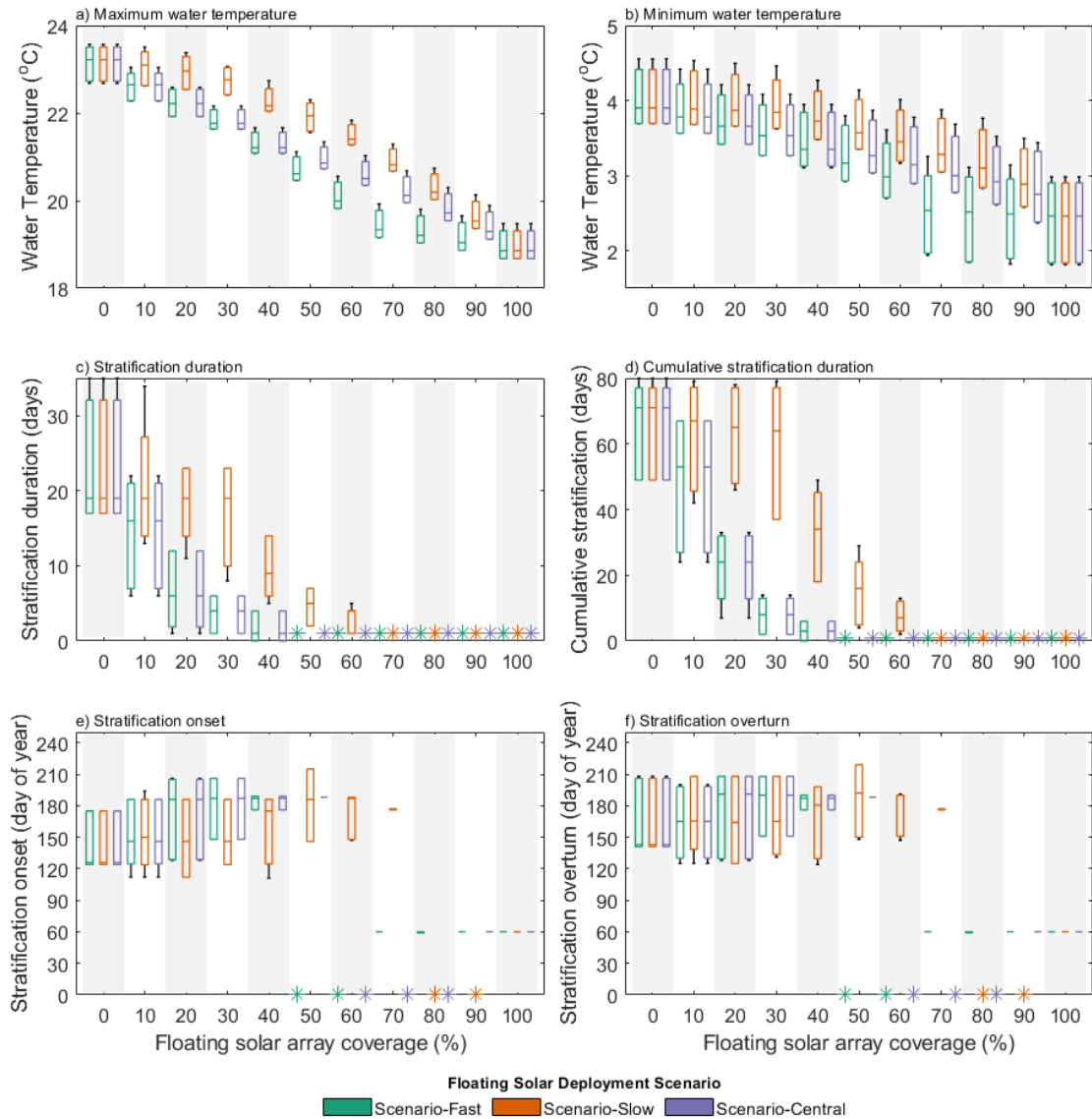
Figure 3 – a) Annual maximum and b) minimum water temperature, c) stratification duration, d) cumulative stratification duration, and stratification e) onset and f) overturn day, versus floating solar (FPV) array coverage for each deployment scenario. An asterisk indicates no prolonged stratification event occurred for the simulation. Whiskers represent the minimum and maximum of the simulation results presented. The box represents the 2.5th & 97.5th percentiles, which gives a 95% confidence interval that simulation estimates fall within this range. 0 % FPV coverage represents QEII reservoir simulated as a baseline with no additional FPV coverage.
