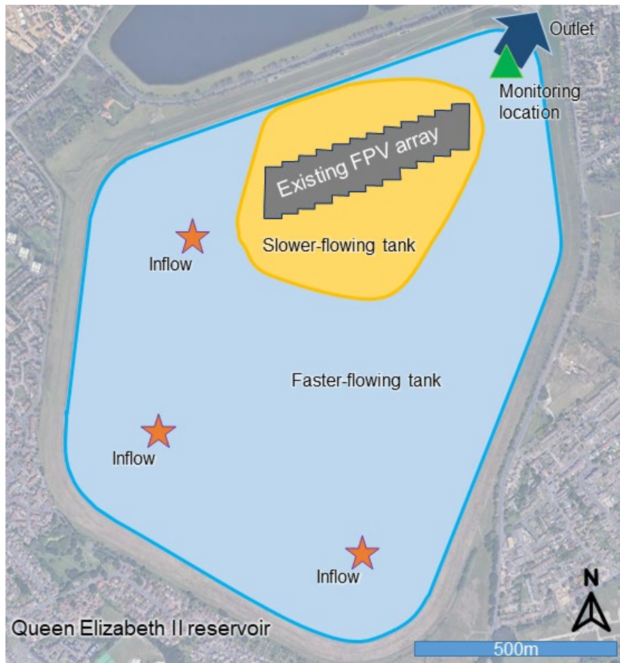
Figure 1 - Conceptual Baseline 'tank' structure for QEII during 2018. Satellite image from Google Earth.
