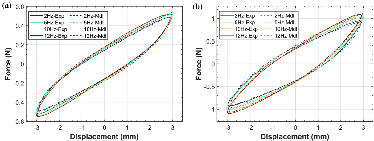
Fig. 12 Hysteretic loops of the actual force (inertial force excluded) for the r_c = 80\% auxetic foam loaded along d_1 (a) and d_3 (b) at different frequencies with an amplitude of 3 mm. Also
