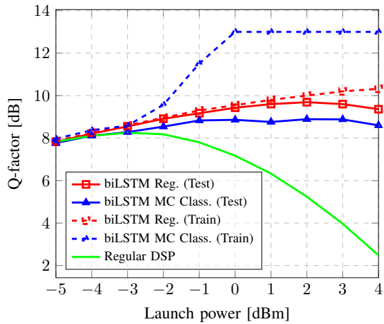
(a) TWC link - biLSTM Equalizer - Q-factor Metric
