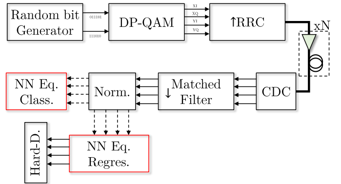
Fig. 6: The schematic of the setup used in our simulations. The two available equalization/soft-demapping types (multi class classification and regression) are inserted at the receiver side after the matching filter and the DSP blocks: CDC and Phase/Amplitude Normalization. The equalizers are highlighted with a red box.
