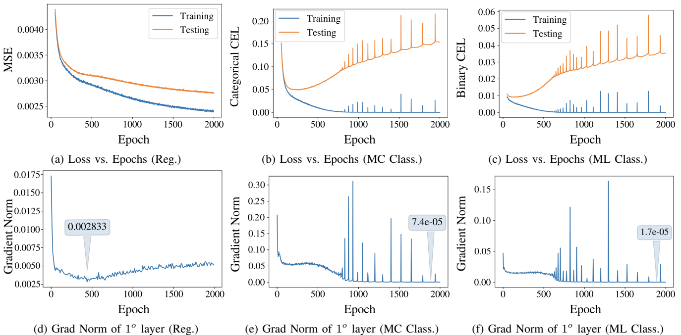
Fig. 12: Overfitting and Gradient Vanishing investigation for the Regression model (a/d), Multi-Class Classifier (MC Class.) (b/e), and Multi-Label Classifier (MB Class.) (c/f).
