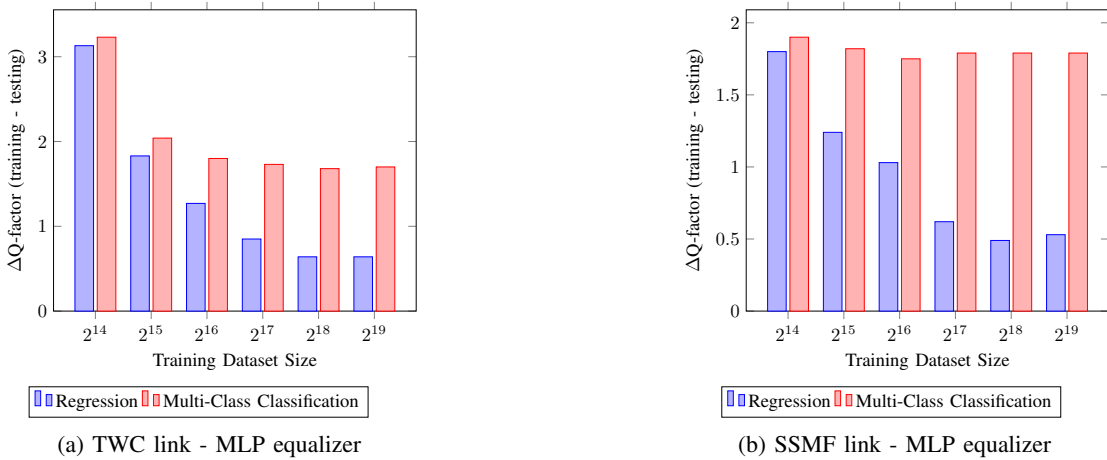
Fig. 10: Difference between training and testing performance over different training dataset sizes to evaluate the overfitting behavior. The MLP was applied for 3dBm 34.4GBd SC-DP, 9x50km TWC and 5x100km SSMF fiber links.
