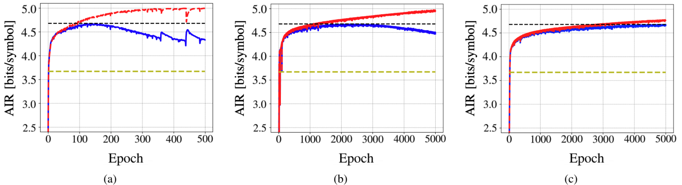
Fig. 9: The performance (AIR) versus training epochs for the 32-QAM SSMF 10 dBm case using the biLSTM Multi-Class Classifier with learning rate equal to (a) 10^{-3} , (b) 10^{-4} , and (c) 5 \times 10^{-5} . The red solid curve is the training performance, the blue solid curve is the test performance, the green dashed line is the reference performance when only the linear equalization is used, and the black dashed line is the reference for the maximum AIR achieved by the testing dataset over the training epochs.
