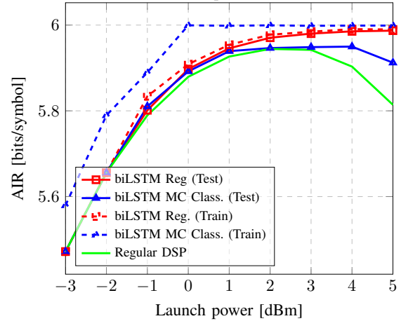
(f) SSMF link - biLSTM Equalizer - AIR Metric
