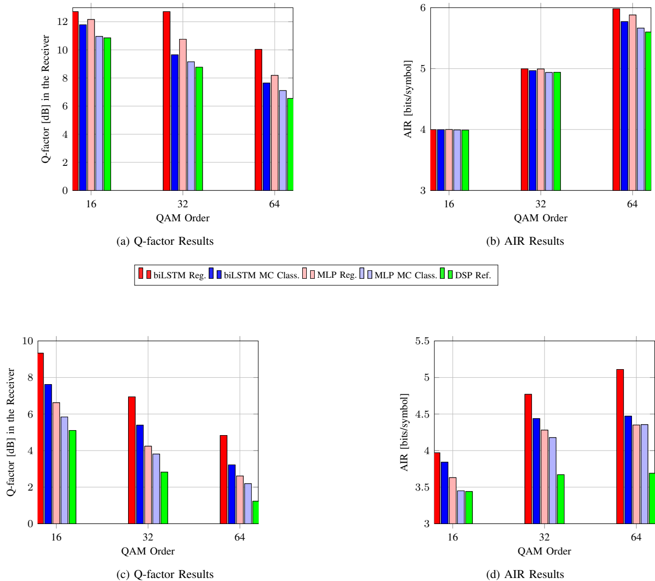
Fig. 7: Performance study for regression equalizer (Reg.) and multi-class classifier (MC Class.) in different modulation format [16-QAM, 32-QAM and 64-QAM] transmission at (a,b) 6 dBm and (c,d) 10 dBm SC-DP, 5x100km SSMF fiber and 34.4G Bd.
