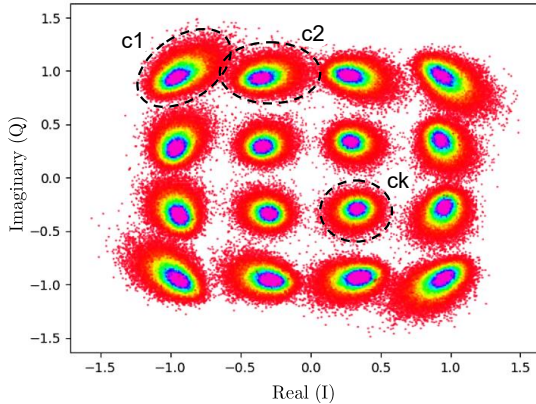
Fig. 4: Distribution of the received symbols in an ideal transmitter of SC-DP 16QAM case with launch power -1 dBm and 34.4 GBd, over 9 \times 50 km TWC fiber. The constellation is given after a standard Rx-DSP described in Sec III.
