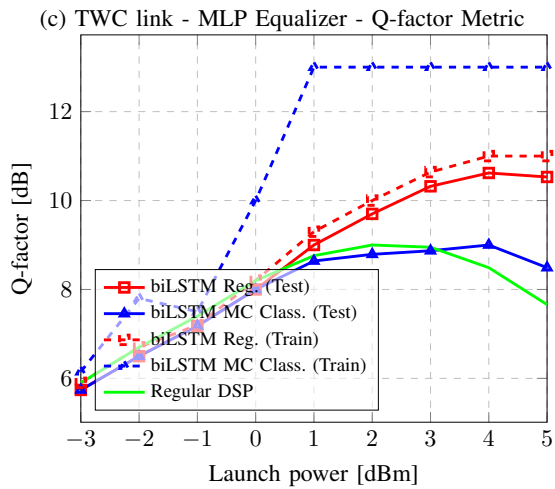
(c) TWC link - MLP Equalizer - Q-factor Metric
