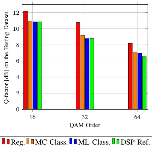
Fig. 13: Performance evaluation on the testing datasets for three different modulation formats (16-,32-, and 64-QAM). The MLP was applied for 6dBm SC-DP, 5 \times 100 km 34.4GBd SSMF fiber links.
