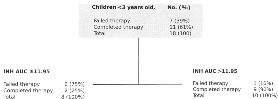
Figure 6. Classification and regression tree (CART) model of predictors of therapy failure in babies and toddlers. The optimal model and variable importance ranking together with the scores for children < 3 years old with failure of therapy. Terminal nodes are shaped as sharp-edged rectangles; intermediate daughter nodes have rounded edges. Abbreviations: AUC, area under the concentration-time curve; INH, isoniazid.
