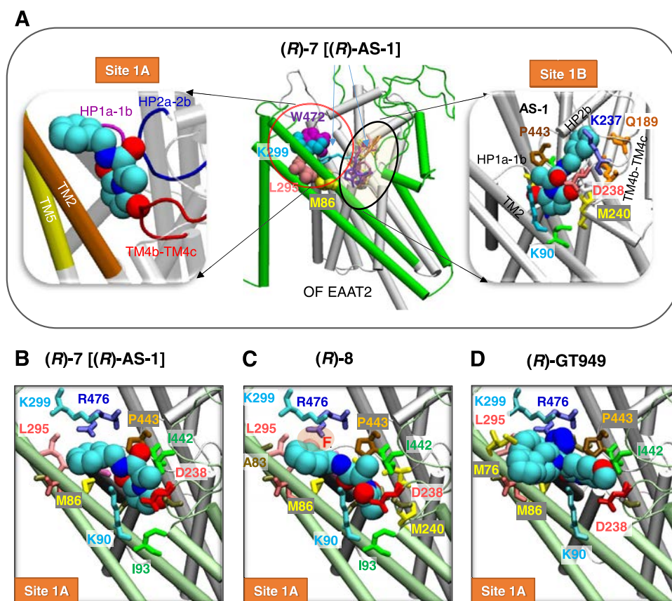
Figure 8. (R) -7 [( R )-AS-1] and (R) -8 bind at the interface between the scaffold domain (green) and the transport domain (white) of human EAAT2 in the OF state. (A) Binding poses of (R) -7 [( R )-AS-1] to the two most favorable sites site 1A and site 1B. The diagram in the center shows the multiple binding poses of (R) -7 [( R )-AS-1] onto OF EAAT2, shown in sticks of different colors. Residues reported earlier to coordinate the binding of PAM (R) -GT949 60 are displayed in van der Waals (VDW) representation in different colors (middle). Site 1A pocket is lined by TM2 (orange) and TM5 (yellow), and the three loops TM4b-4c (red), HP1a-1b (purple), and HP2a-2b (blue) (left) and site 1B pocket is lined by residues from TM2, TM4b-4c, HP1a-1b and HP2 (right). Site 1A and site 1B, shown on the left and right panels, are predicted to show equal affinity ( -7.3 kcal/mol). (B–D) Comparison of the predicted binding poses of (R) -7 [( R )-AS-1] (B), (R) -8 (C), and (R) -GT949 (D) onto site 1A. AutoDock predicts the respective binding affinities of the three compounds to site 1A as -7.3 , -7.6 , and -8.0 kcal/mol. The EAAT2 protein was modeled after the EAAT1 OF conformer (PDB: 5LLU).
