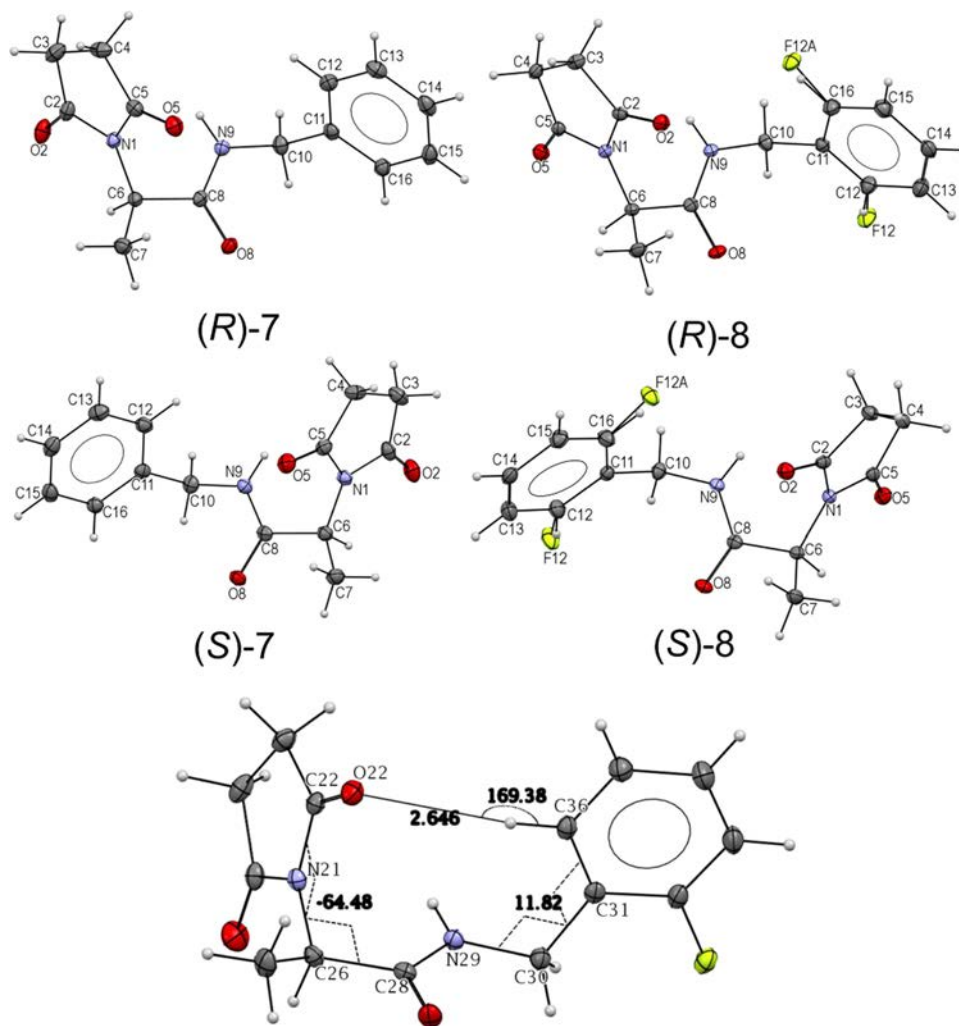
Figure 2. Molecular geometry observed in the crystal structure of enantiomeric pairs (R)-7 [(R)-AS-1], (S)-7 and (R)-8, (S)-8 (only one molecule from the asymmetric unit is shown for figure clarity, presenting the numbering scheme). Below, the distinct molecular geometry observed in structure (R)-8 (similar also for (S)-8) that results from the formation of the intramolecular hydrogen bond C36–H···O22 stabilizing the preferential conformation.
