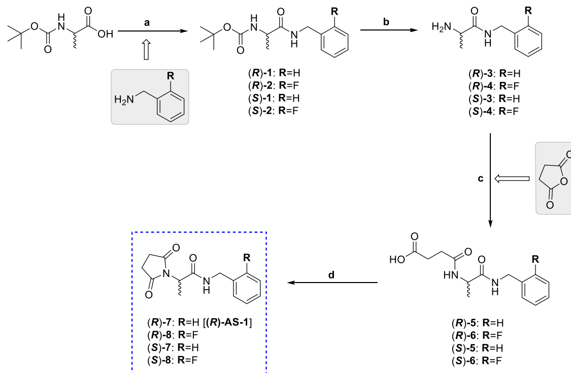
Scheme 1. Synthesis of Target Enantiomers ( R )-7 [( R )-AS-1], ( R )-8, and ( S )-7, ( S )-8 a
