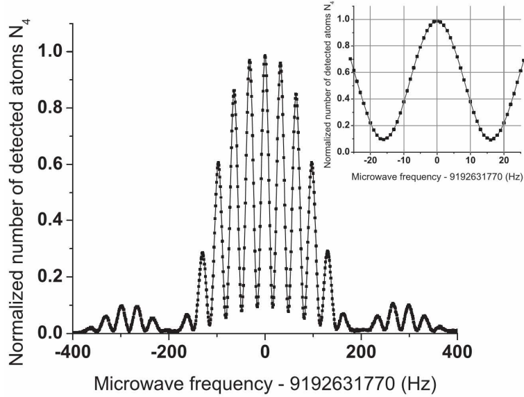
Fig. 25. – Ramsey fringes observed in HORACE; the inset shows the central fringe of the Ramsey pattern. N_4 is the number of detected atoms in level |F = 4, m_F = 0\rangle . Reprinted figure with permission from: F. -X. Esnault, D. Holleville, N. Rossetto, S. Guerandel and N. Dimarcq N., Phys. Rev. A 82,033436, 2010. Copyright 2012 by the American Physical Society.
