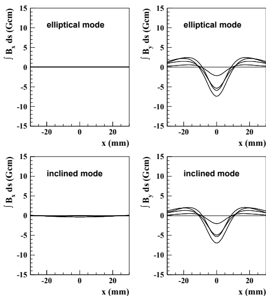
Figure 2: Evaluated field integral variations with phase at 15 mm gap (magnet size 40 x 40 mm 2 ).
