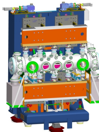
Figure 4: CPMU-17 undulator.
