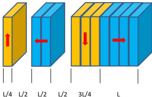
Figure 1: End-pole configuration.
