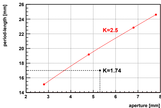
Figure 5: Red: Minimum period length which provides K=2.5 at a given aperture (magnetic gap - 0.2mm). By design the CPMU-17 value lies below this curve.
