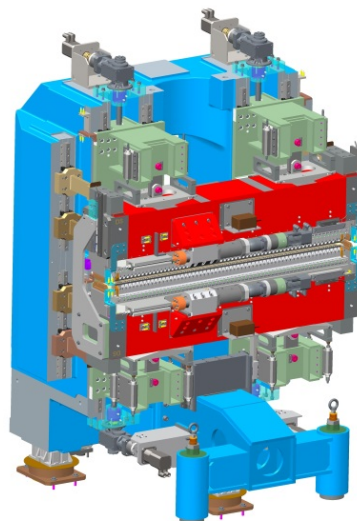
Figure 3: UE-48 APPLE II undulator.
