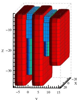
Figure 6: Endpole configuration of the CPMU-17 (RADIA coordinate system). The last magnet (red) and the last pole (blue) can be adjusted vertically.
