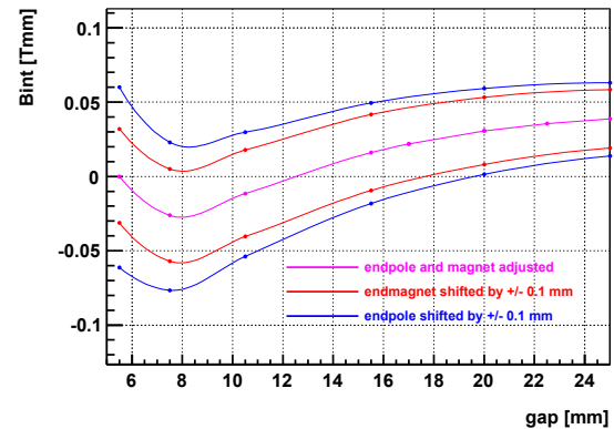
Figure 7: First field integral of the CPMU-17 endpole structure.
