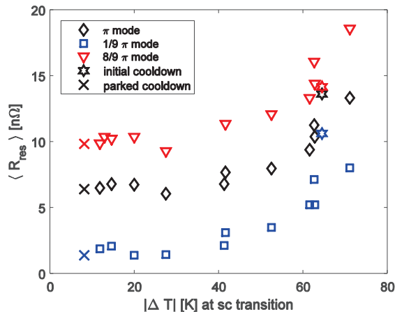
Figure 3: R_{\text{res}} measured with the three passband modes as a function of \Delta T along the cavity at the onset of sc phase transition. The lowest R_{\text{res}} was achieved in the center cells following the cycle 1 and the parked cooldown.
