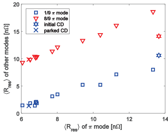
Figure 4: R_{\text{res}} obtained for the 8/9\pi and 1/9\pi mode as a function of R_{\text{res}} obtained for the \pi mode.
