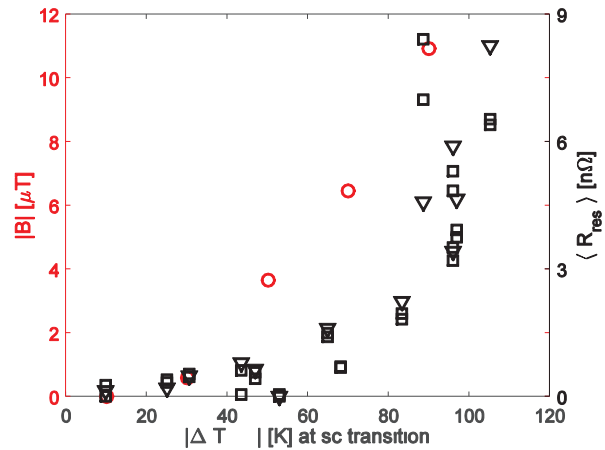
Figure 5: Magnetic field at the RF surface simulated in COMSOL for different temperature differences in combination with the RF data of Figure 3 (change in residual resistance).
