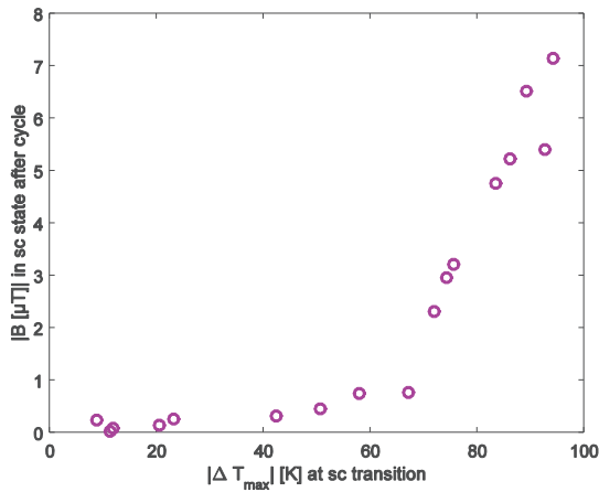
Figure 7: Trapped flux in the superconducting state at the RF surface.
