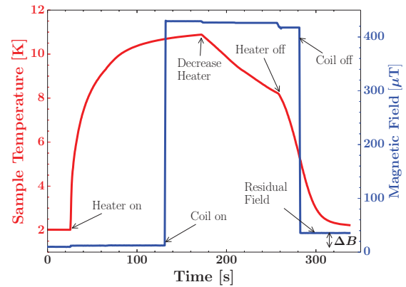
Figure 9: Sample temperature and reading of flux-gate magnetometer during thermal cycle with field cooldown.
