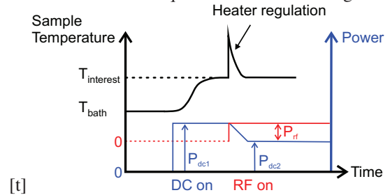
Figure 2: Illustration of the measurement principle. [8]
