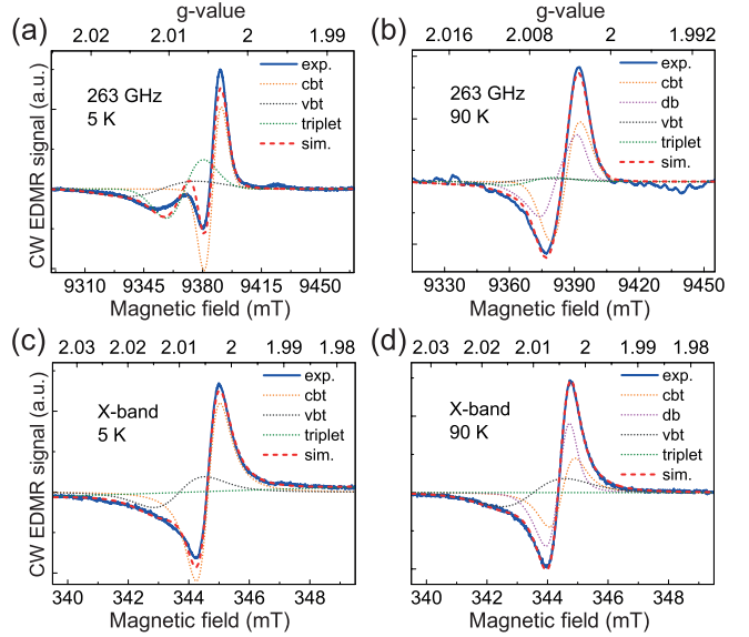
Figure 4: (color online). Experimental (solid blue) and simulated (red dashed) CW EDMR spectra. 5K (a) 263 GHz and (c) X-band EDMR spectra were simulated assuming a superposition of isotropic cbt ( g = 2.0044 , g -strain = 0.0025, field independent Lorentzian line width = 1 mT), vbt ( g = 2.011 , g -strain = 0.01, field independent Lorentzian line width = 1.5 mT) and triplet ( g = 2.008 , field independent Gaussian line width = 26 mT) signals. 90 K (b) 263 GHz and (d) X-band EDMR spectra were simulated assuming identical g -values and line shape parameters for cbt, vbt and triplet states and an additional db ( g_{xx} = 2.0079 , g_{yy} = 2.0061 and g_{zz} = 2.0034 , g_{xx} -strain = 0.0054, g_{yy} -strain = 0.0022, g_{zz} -strain = 0.0018, field independent Voigtian line of 0.13 mT Gaussian and 0.43 mT Lorentzian line width) contribution. Dotted orange, black, magenta and green lines represent contributions from cbt, vbt, db and triplet states, respectively.
