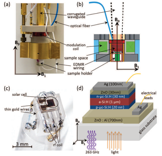
Figure 2: (color online). (a) Photograph and (b) cross section of the 263 GHz EDMR probe. (c) Photograph of the EDMR sample holder with mounted a-Si:H p-i-n solar cell. The radio frequency (rf) coils shown in the figure can be used for rf excitation of the sample. (d) Layer structure of the a-Si:H p-i-n solar cell. B_0 and B_1 indicate the constant external magnetic field and the magnetic component of the mw field, respectively.
