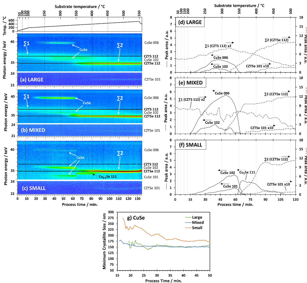
Fig. 2 Left: Subsection of the slow ramp EDXRD data for (a) large, (b) mixed, and (c) small particle films showing the occurrence of \Sigma 1 , \Sigma 2 , \text{CuSe} , and \text{Cu}_{2-6}\text{Se} diffraction peaks in the film. Peak assignments for \text{CuSe} were made based on ICDD card 086-1240). See SI for full data range. Right: Evolution of integrated peak intensities for slow heating of (d) large, (e) mixed, and (f) small particle films. Bottom: (g) Minimum crystallite size ( D/k ) as described in Ref. 13 estimated using the most intense peak in each sample for \text{CuSe} (i.e. 006 planes for large and mixed particle films, 102 planes for small precursor film) during slow heating.
