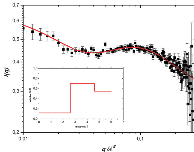
Fig. 4 SANS profile of deuterated ACE-16 in protonated toluene. The red line shows a fit of a spherical core shell structure with 9.2 Å diameter. Inset: the corresponding spherical core shell model with relative neutron SLD (scattering length density profile), normalised to the SLD of the solvent.
