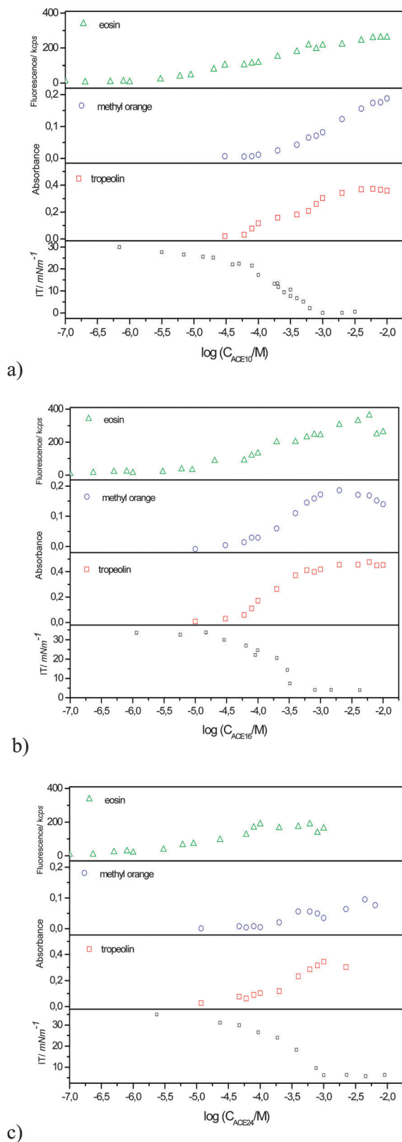
Fig. 3 ACE concentration dependence of absorbance (methyl orange, \lambda_{max} = 414 nm and tropeolin OO, \lambda_{exc} = 408 nm) and emission (eosin Y, \lambda_{exc} = 310 nm, \lambda_{em} = 558 nm) of the toluene phase for (a) ACE-10, (b) ACE-16 and (c) ACE-24. The interfacial tension isotherms are reproduced from ref. 10.
