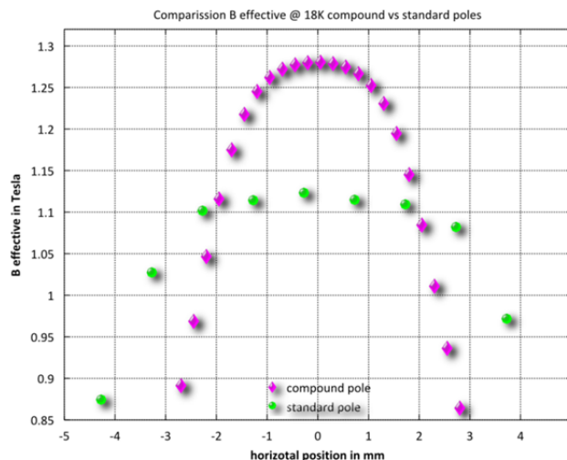
Figure 4: Comparison of results from field measurements.
