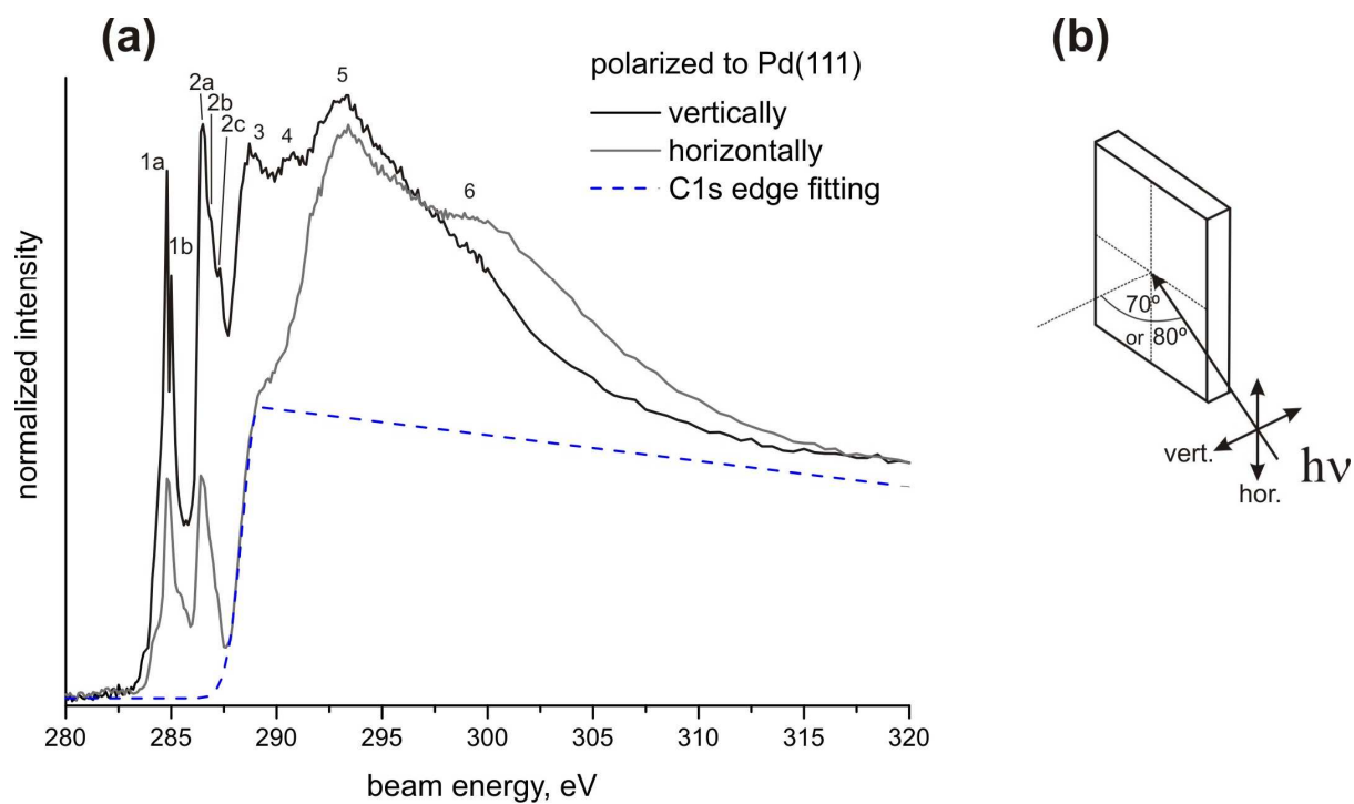
Figure 4: (a) C K edge NEXAFS of 0.7 ML isophorone / Pd(111) at 100 K in vertical and horizontal polarization. The spectra are normalized to the C K edge, which was fitted and is indicated with the dashed line. The most pronounced transitions around the edge are indicated with numbers 1 to 6. The assignment is given in Table 1. (b) Schematic representation of the NEXAFS experimental geometry.
