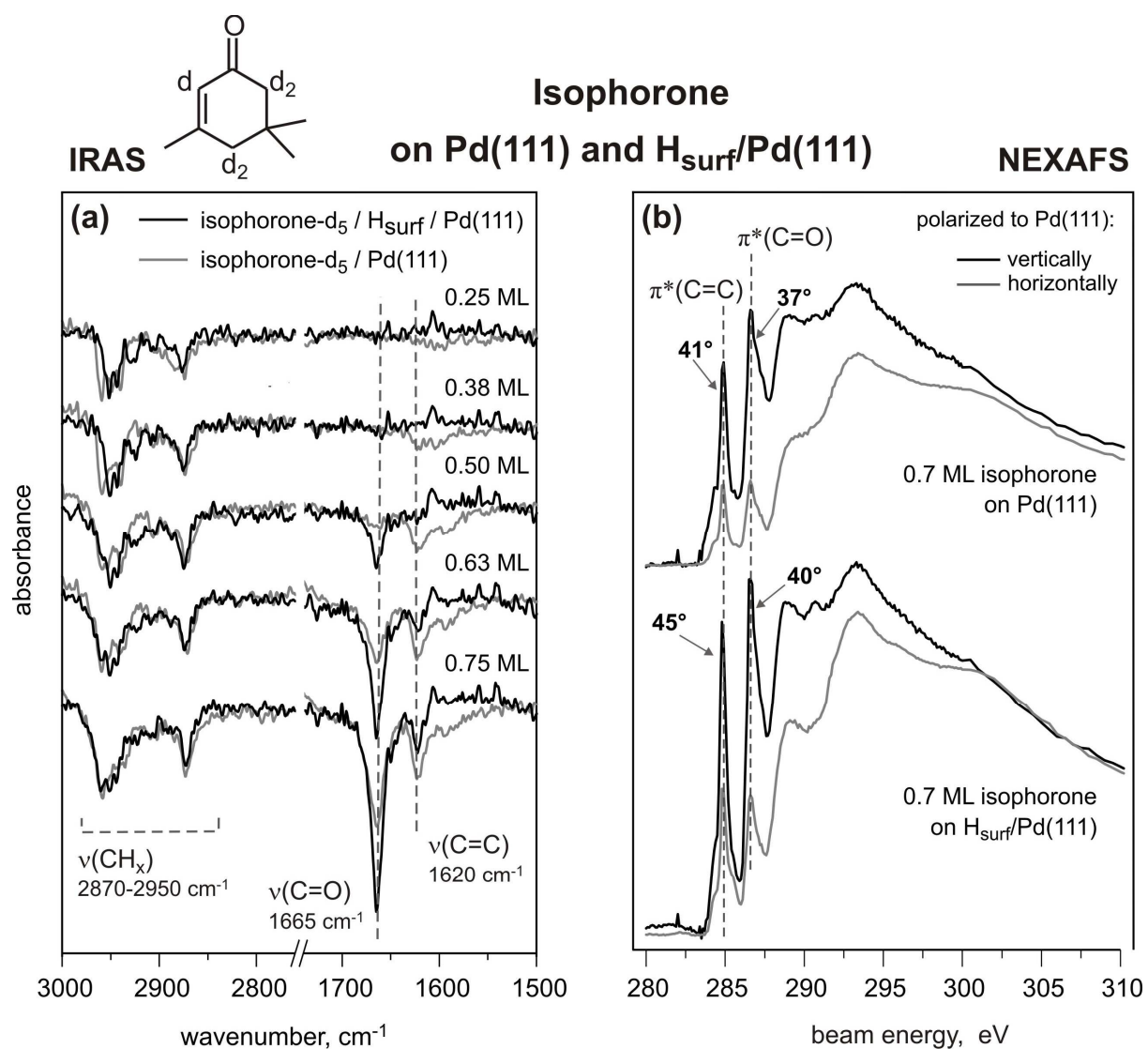
Figure 6: (a) IR spectra of d 5 -isophorone adsorbed at 100 K on hydrogen pre-covered (black traces) and pristine (grey traces) Pd(111) for different exposures. Displayed are two main vibrations regions: from 3000 to 2750 cm -1 (C-H stretching vibrations) and from 1750 to 1500 (C=O and C=C stretching vibrations). (b) NEXAFS spectra obtained at 100 K for 0,7 ML isophorone coverage on pristine Pd(111) (upper traces) and H pre-covered Pd(111) (lower traces).
