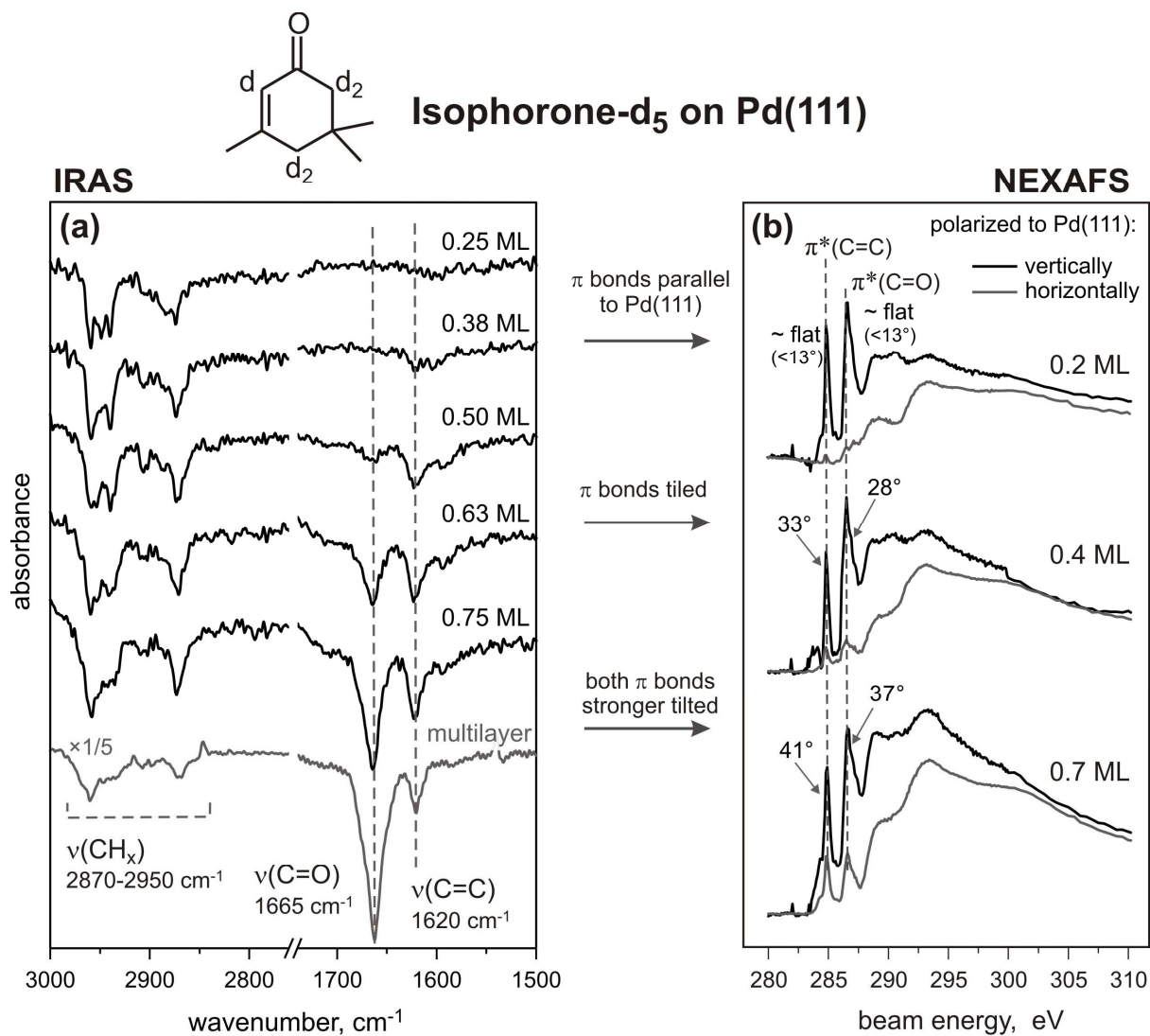
Figure 3: (a) IR spectra of d 5 -isophorone adsorbed at 100 K on pristine Pd(111) for different exposures displayed for two main vibrations regions: from 3000 to 2750 cm -1 (C-H stretching vibrations) and from 1750 to 1500 (C=O and C=C stretching vibrations). (b) NEXAFS spectra of isophorone/Pd(111) obtained at 100 K show coverage dependent orientations of both π bonds.
