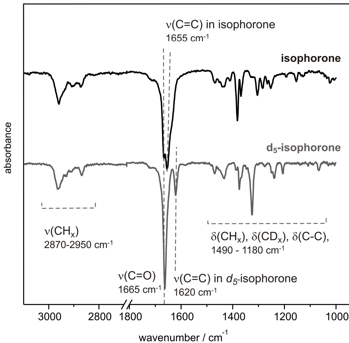
Figure 2: IR spectra of isophorone ice for regular (upper trace) and d_5 -substituted form formed at 100 K on Pd(111). Three main spectral regions can be distinguished characteristic for C-H stretching (2800 – 3200 cm -1 ), C=C and C=O stretching (1550–1850 cm -1 ) and for C-H, C-D and C-C deformation vibrations (< 1500 cm -1 ).
