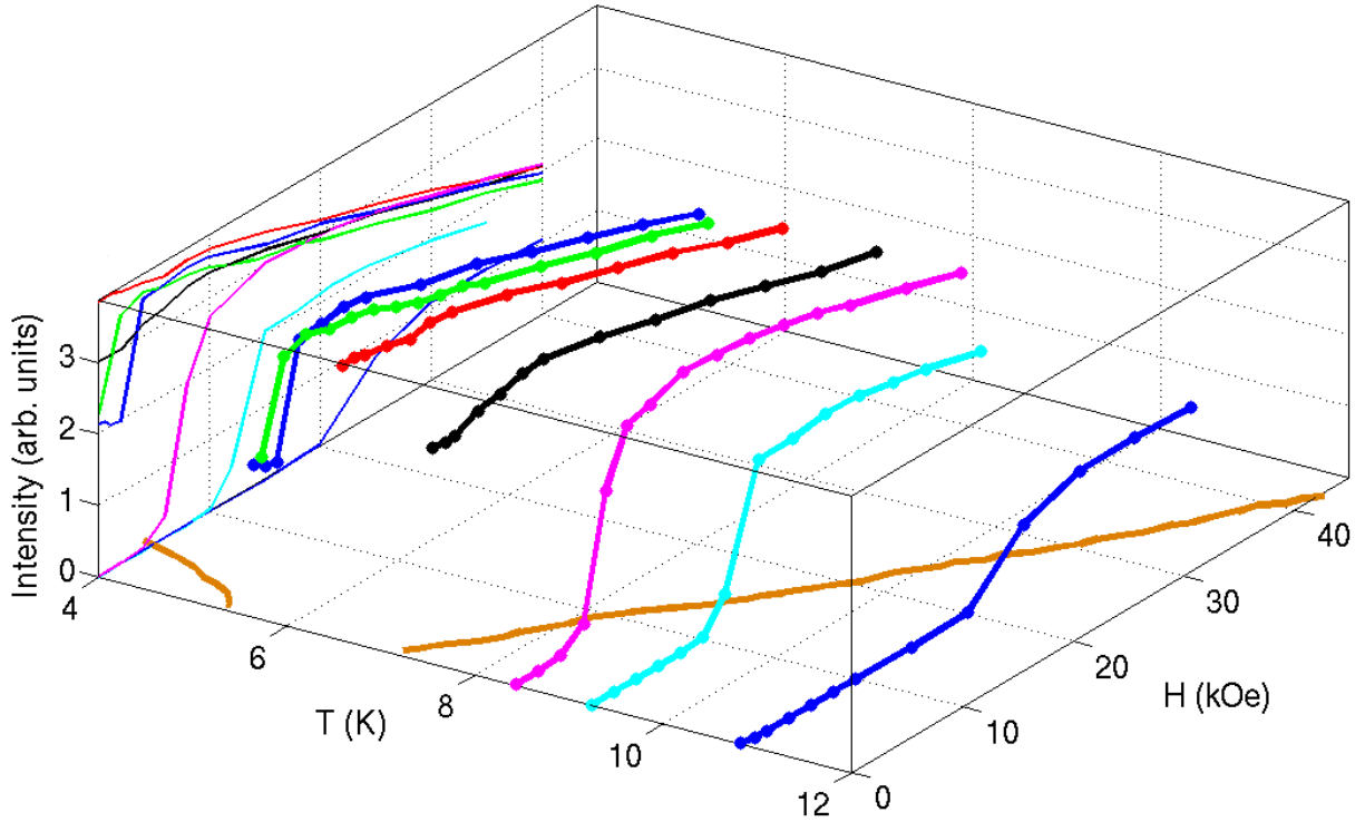
Figure 2. Field dependences of the (0 \frac{1}{4} 6) integrated intensity as function of \mathbf{H} \parallel \mathbf{b} at fixed temperatures, with projections. The orange curves represent the boundaries of the ferroelectric phase from the phase diagram in [4].
