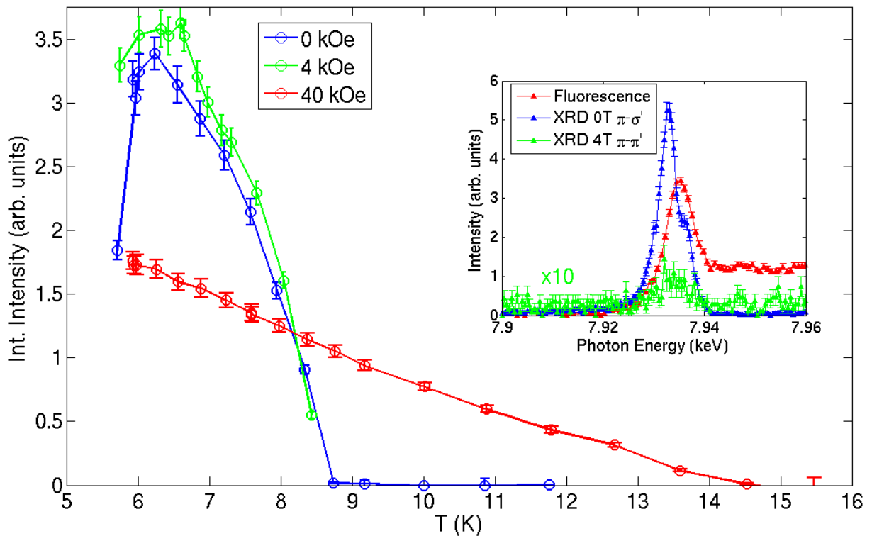
Figure 1. Temperature dependence of the (0 \frac{1}{4} 6) integrated intensity at different field values. The inset shows the energy dependence across the Gd L_2 edge at T = 5.7 K, in zero field in \pi - \sigma' as well as high field in \pi - \pi' , along with a fluorescence measurement of the sample.
