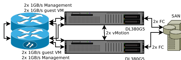
Figure 1: HP DL380G5 cluster
