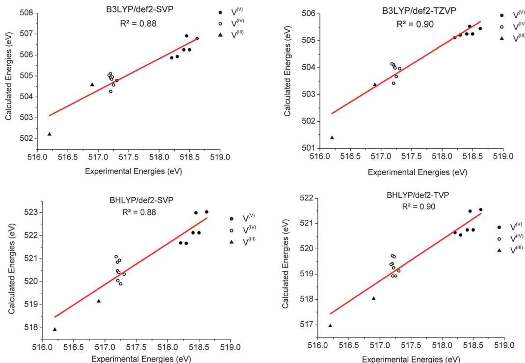
Fig. 4 Relationship of calculated versus experimentally determined transition energies for B3LYP/def2-SVP (upper left), B3LYP/def2-TZVP(-f) (upper right), BHLYP/def2-SVP (lower left) and BHLYP/def2-TZVP(-f) (lower right). The linear least-squares fits are given by f^{\text{B3LYP/def2-SVP}} = 1.50(\text{exp}) - 275.54 eV, f^{\text{B3LYP/def2-TZVP(-f)}} = 1.40(\text{exp}) - 224.22 eV, f^{\text{BHLYP/def2-SVP}} = 1.77(\text{exp}) - 397.54 eV and f^{\text{BHLYP/def2-TZVP}} = 1.63(\text{exp}) - 326.91 . The notation exp refers to experimental values in eV.
