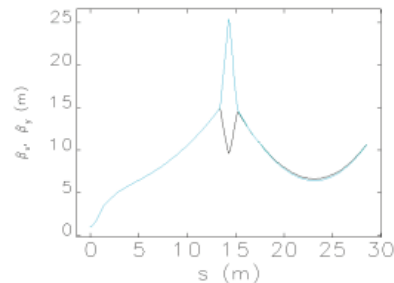
Figure 5: Optics design of the preinjection linac.
