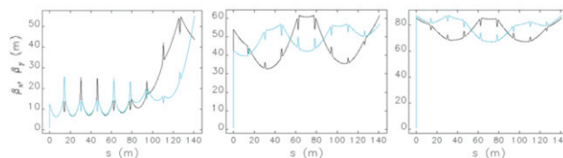
Figure 8: Optics design of the first 0.96 GeV linac. 3 passes on acceleration are presented from left to right.
