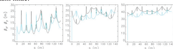
Figure 9: Optics design of the second 0.96 GeV linac. 3 passes on acceleration are presented from left to right.
