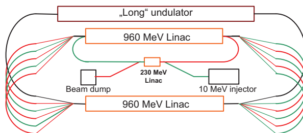
Figure 7: New scheme of a scalable FSF.
