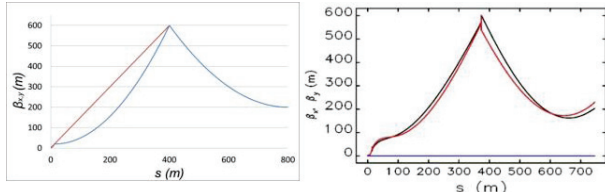
Figure 3: Theoretical (left) and calculated in Elegant program optics design of the beta-functions in the main linac for the direct injection scheme.
