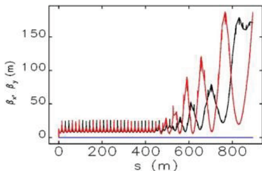
Figure 6: Optics design of the main 6 GeV linac for the two stage injection scheme.
