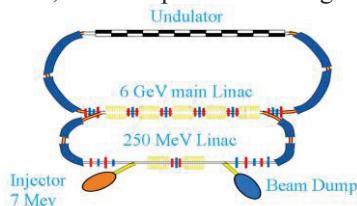
Figure 4: Two stage injection scheme.
