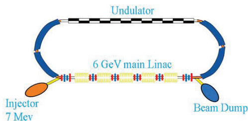
Figure 1: Direct injection scheme.
