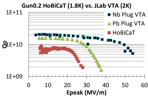
Figure 4. The Q vs. E_{\text{peak}} curve of Gun0.2 taken in HoBiCaT at 1.8 K compared to the data from the JLab VTA at 2K.
