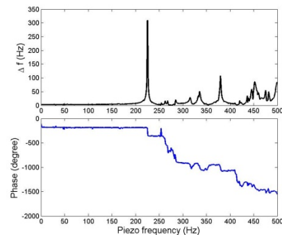
Figure 5. Piezo tuner to cavity detuning transfer function.
