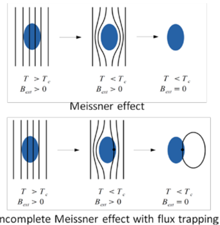
Figure 2: Meissner effect with flux trapping
