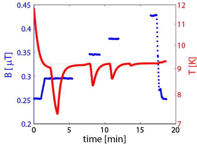
Figure 6: Manual expulsion of frozen flux from a superconducting rod by heating below T_c . The absolute value of B increases because flux is driven out of the rod increasing the measured flux density at the sensor position. Once, T_c is exceeded flux re-enters the sample reducing the measured value at the sensor position.
