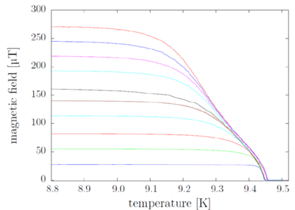
Figure 5: Flux release of different levels of trapped magnetic field in a single crystal Niobium sample (BCP + 1200°C) upon heating in zero external field.
