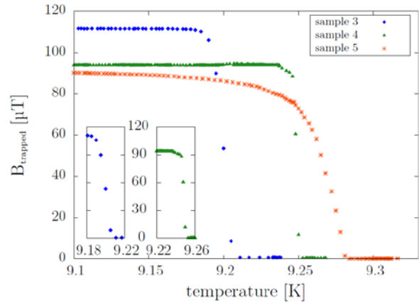
Figure 4: Flux release as a function of sample preparation history. Polycrystalline, BCP treated and post annealed at 800°C (blue squares); single crystal, BCP treated (green triangles); single crystal, BCP treated and post annealed at 800°C (red crosses). The time step between two neighbouring points is 1 sec. Note that slightly different field levels were applied and the thermo sensors had slightly different offsets.
