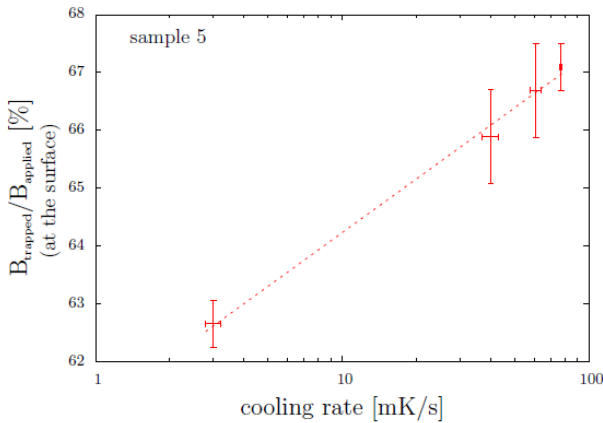
Figure 3: Dependence of the trapped field on the cooling rate for a single crystal sample with 800°C tempering.
