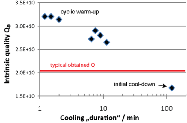
Figure 1: Dependence of obtained Q_0 on cool-down speed. Measurements were taken at 1.8K and E_{\text{acc}} = 4 \text{ MV/m} .
