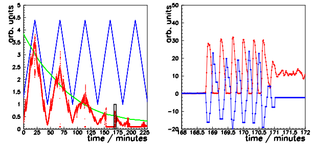
Figure 3: Rf-voltage scans and THz signals as a function of time (horizontal axis). Left: THz signals (red), rf-voltage (blue) and beam current (green). The data inside the small black box are shown in the right part of the figure: horizontal orbit position (blue) and THz signal intensity (red) are oscillating during the voltage scan.
