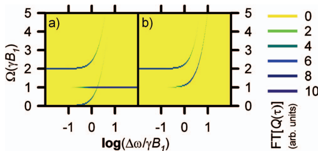
FIG. 3. (Color) Color plot of the Rabi-frequency components \Omega = \text{FT}\{Q(\tau)\} as function of \log(\frac{\Delta\omega}{\gamma B_1}) for an excitation frequency (a) \omega = \omega_{a,b} on resonance with one of the pair partners and (b) \omega = \omega' on resonance with the average \omega' of the pair partners Larmor frequencies.
