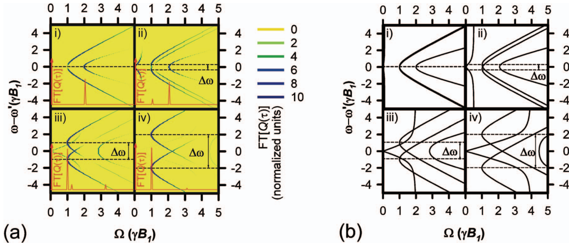
FIG. 2. (Color) (a) Three-dimensional color plots of the semianalytically calculated \Omega = \text{FT}\{Q(\tau)\} as a function of the excitation frequency \omega scaled in units of \gamma B_1 as the difference between \omega and the average of the Larmor frequencies of the two pair partners \omega' = \frac{1}{2}(\omega_a + \omega_b) and the Rabi-nutation frequency \Omega in units of \gamma B_1 . For all four plots (a.i) to (a.iv), \frac{\gamma}{2}B_1 = 10 MHz and \frac{\omega'}{2\pi} = 10 GHz. From plot (a.i) to (a.iv), the Larmor separation increases: (a.i), \frac{\Delta\omega}{2\pi} = 1 MHz; (a.ii), \frac{\Delta\omega}{2\pi} = 5 MHz; (a.iii), \frac{\Delta\omega}{2\pi} = 20 MHz; (a.iv), \frac{\Delta\omega}{2\pi} = 40 MHz. The two-dimensional inset plots display the data of the three-dimensional plot at the Larmor frequency slices indicated by the dashed lines. (b) The plot of the Rabi-nutation frequencies as obtained from Eqs. (3) and (4) for the same parameters as used for the calculated results in (a). A comparison with the frequencies therein shows an excellent agreement.
