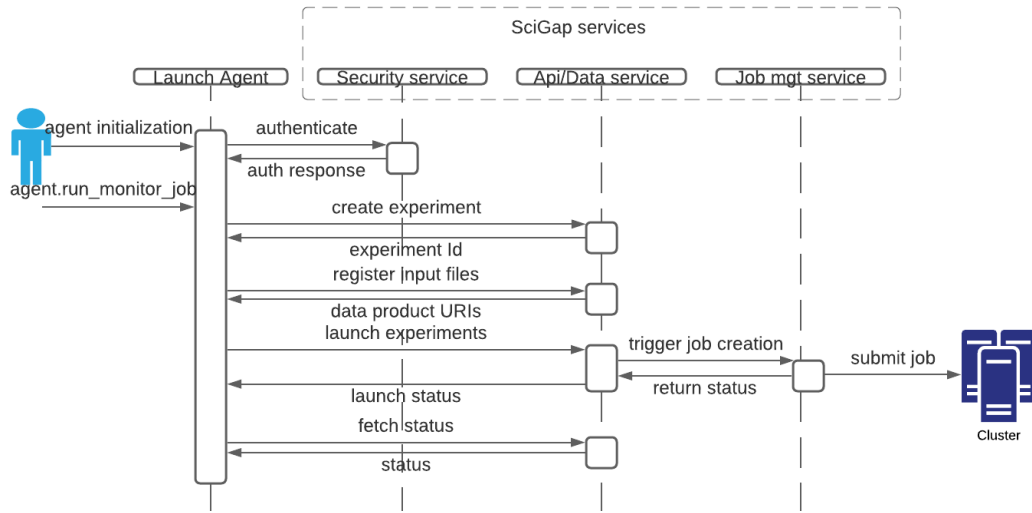
Fig. 5: LaunchAgent Operation Sequence with SciGaP services.
