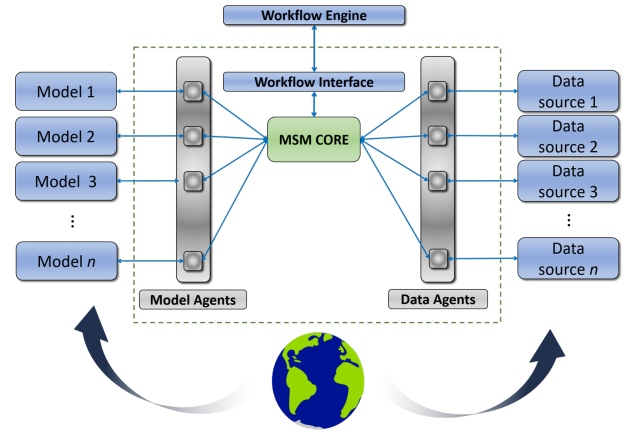
Fig. 1: Broad Scheme of CyberWater.
