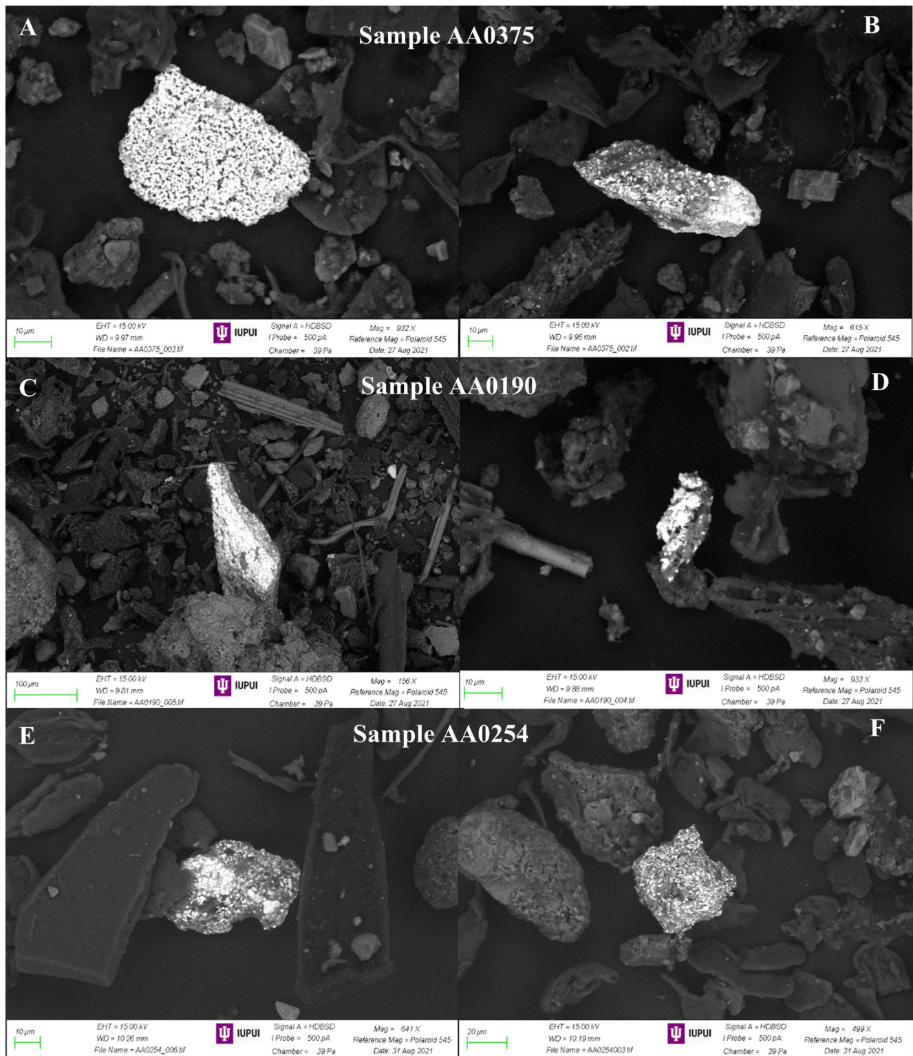
Figure 5. Scanning electron microscopy images of particles resembling Pb paint, surrounded by other particulates in various high Pb DustSafe household dust samples (corresponding dispersive X-ray spectroscopy spectra provided in Figures S5–S10 in Supporting Information S1). Pb paint particles are evident by very high contrast of electron backscatter detection—more so than surrounding particles because of the high atomic number of Pb. Most Pb-bearing particles are angular or jagged, with clear flaky particles on their surface.
