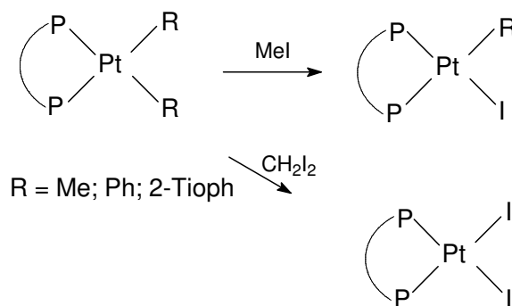
Figure 4. The synthesis of Pt\{(S,S)\text{-BDPP}(I)(R) ( R = \text{Me}, \text{Ph}, 2\text{-Tioph} ) complexes
