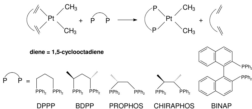
Figure 2. The ligand-exchange reaction of platinum-dimethyl-COD-complex and the diphosphine ligands used
