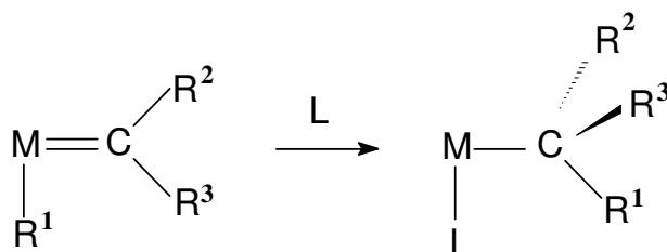
Figure 1. The formation of an asymmetric centre via the insertion of a carbene
