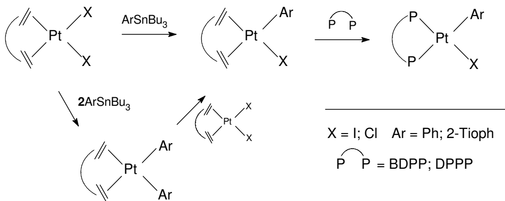
Figure 3. The synthesis of Pt(PP)(X)(\text{alkyl/aryl}) complexes
