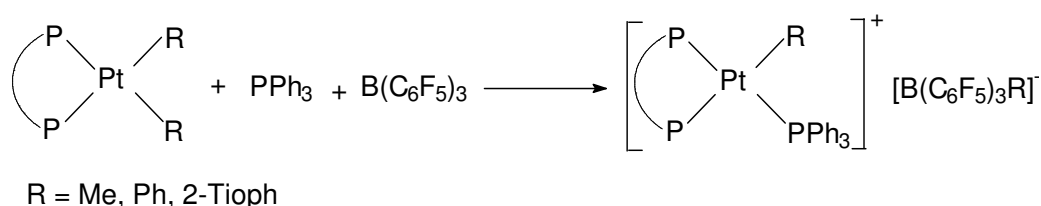
Figure 7. The formation of [\text{Pt}(\text{BDPP})(\text{PPh}_3)(\text{alkyl/aryl})]^+ complexes
