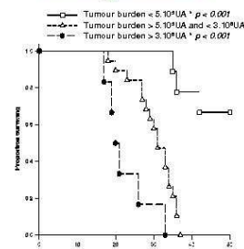
(fig. 2) Variability in response with 500µg of rituximab.
