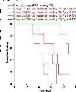
(fig. 3) Tumour burden and disease response.
