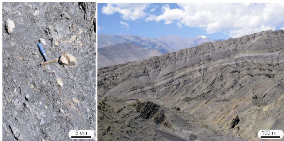
Pebbly mudstone with C2 age Late Triassic terrigenous rocks unconformably overlying on the Late Permian rocks
