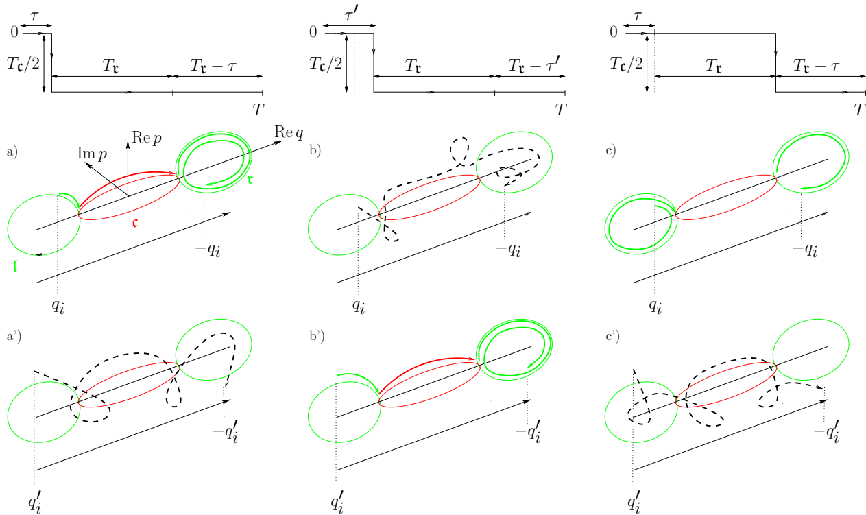
Figure 3: (colour online) For the double well in Fig. 1, at a given energy 0 < E < V_{\max} , when T = 2T_c(E) - iT_c(E)/2 , for each one-step time path, there exists a unique half symmetric periodic orbit with energy E keeping \text{Im } q = 0 starting from the left allowed region. Its initial point is uniquely defined: For the time-path depicted in the left column, (p_i, q_i) is such that it takes exactly the real time \tau to reach the turning point (0, -q_r) following the primitive orbit l . Then it follows half of the orbit c and ends in the right well winding once along \tau (a). When starting at q'_i < q_i , there still exists a half periodic orbit joining (p'_i, q'_i) to (-p'_i, -q'_i) in time T for some p'_i but unlike the previous one it gets outside the three dimensional section \text{Im } q = 0 (its projection is schematically represented by the dashed line in a'). However an appropriate shift of the time step to \tau' > \tau (central column) turns the latter smoothly into a trajectory with \text{Im } q = 0 (b'). During this process, the first trajectory starting at q_i cannot keep a purely real q anymore (b). If we shift the step by exactly T_c (right column), we recover a trajectory starting at q_i with purely real q (c) but with a different topology since it is now winding once along l . The change of topology occurs when the initial position reaches a turning point while sliding the step.
