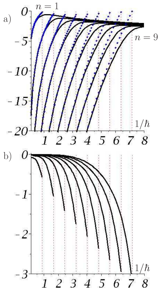
Figure 5: For the pendulum with \gamma = 1 , we have plotted in a) the exact value of \ln(\Delta_n) (see eq. (47)) versus 1/\hbar for n = 1, \dots, 9 (black lines). The dots are given by the semiclassical approximation \ln(\Delta_n) (see eq. (58b)) up to the maximum value of 1/\hbar (vertical dotted lines) where E_n^+ become lower than the separatrix energy \gamma . The semiclassical limit is obtained when the states become more and more localised in the region of phase space corresponding to rotations: for a fixed n this requires to increase E_n \simeq n^2\hbar^2/2 that is to increase \hbar ; or for a fixed energy E > \gamma , we must increase n \propto \sqrt{2E}/\hbar . To control the validity of the prefactors, we can check in b) that \ln(\Delta_n/\Delta_n) approaches zero in the semiclassical limit.
