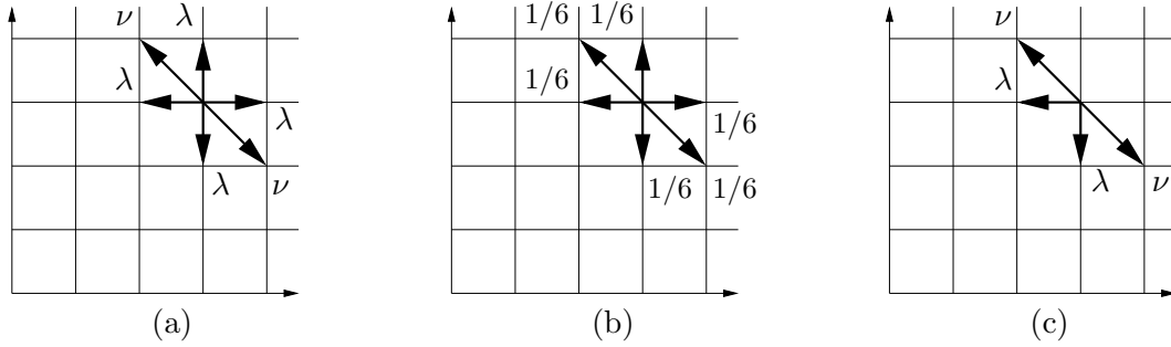
FIGURE 1. Walks considered in [16], [2] and [9], respectively
