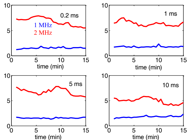
Figure 12: Pulse Peak Time Average Intensity ( \text{W/cm}^2 ) measured for long CW excitation versus time. Duty cycle is 50 % and burst period 0.2, 1, 5 and 10 ms. V_0 = 70 \text{ V} , V_{pp} = 60 \text{ V} .
