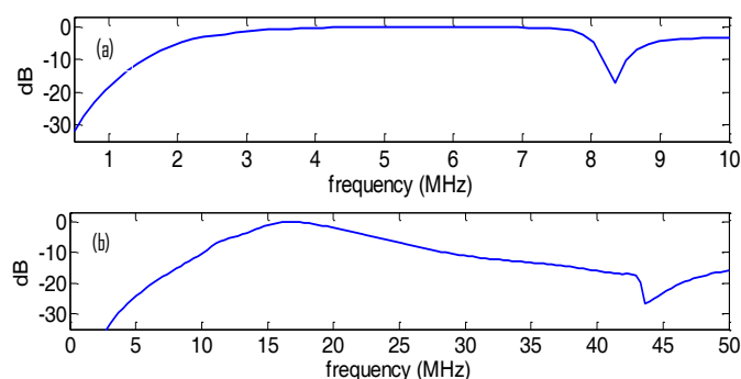
Figure 8: Theoretical pressure spectrum emitted by LF (a) and HF (b) arrays.
